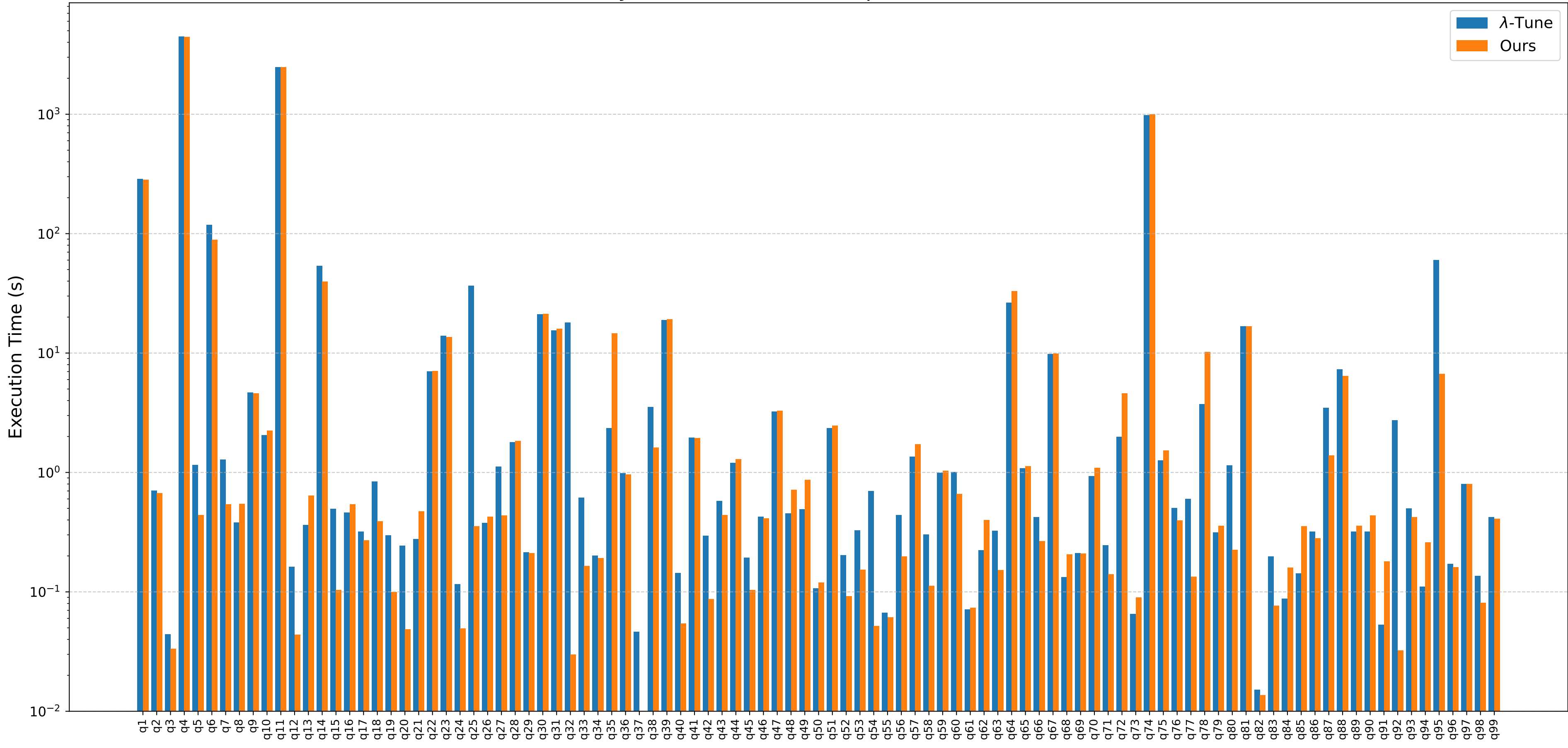
Query Execution Time Comparison for TPC-DS
