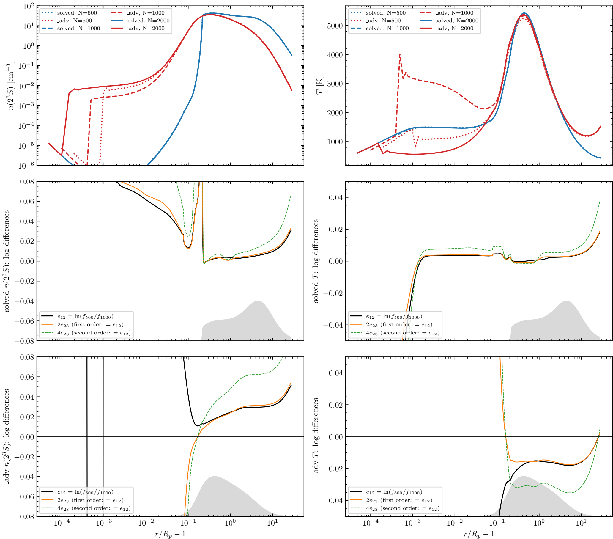
He/H = 1.6: three grids (top) and grid differences (grey: weight n(2^3S)r of the finest grid)
