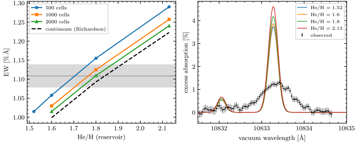
Figure 1: Left: the red-pair EW of the certified molecular states against the reservoir He/H on 500, 1000 and 2000 cells and in the continuum limit, with the observed 1.108 \pm 0.030 \% \text{ \AA} (grey). Right: the unbroadened 500-cell spectra against the released one.
