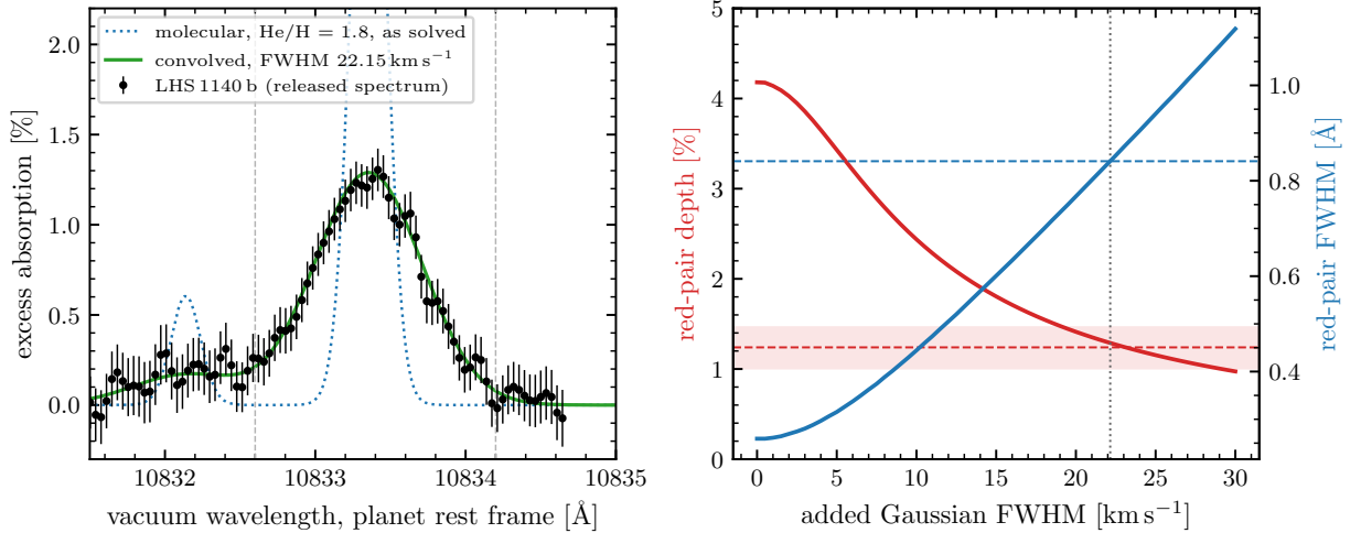
Figure 2: Left: the molecular He/H = 1.8 profile as solved (dotted) and convolved with a 22.15 \text{ km s}^{-1} FWHM Gaussian (solid), against the released spectrum; both model curves are shifted by the memo's v_{\text{wind}} = +2.26 \text{ km s}^{-1} for display (every EW is from the unshifted arrays), and the dashed verticals mark the EW window. Right: the red-pair depth (red, left axis) and FWHM (blue, right axis) as the added Gaussian is scanned; dashed lines are the observed values, the band the 1\sigma interval of the fitted depth, and the dotted vertical the matched kernel.
