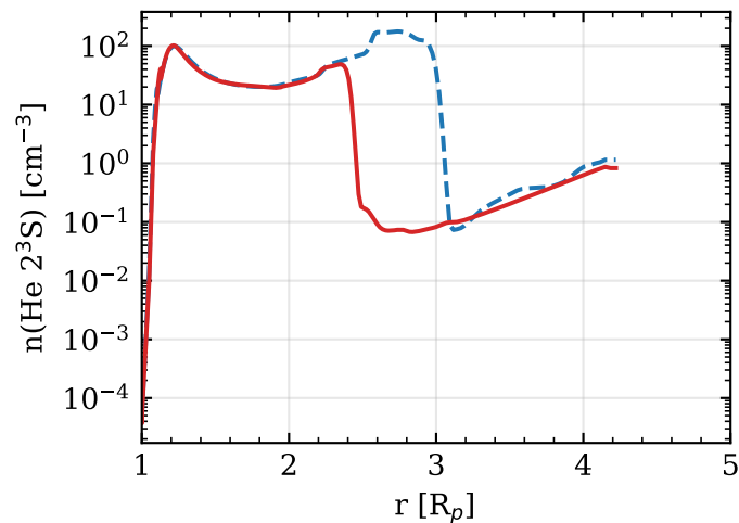
metastable He 2^3\text{S}
