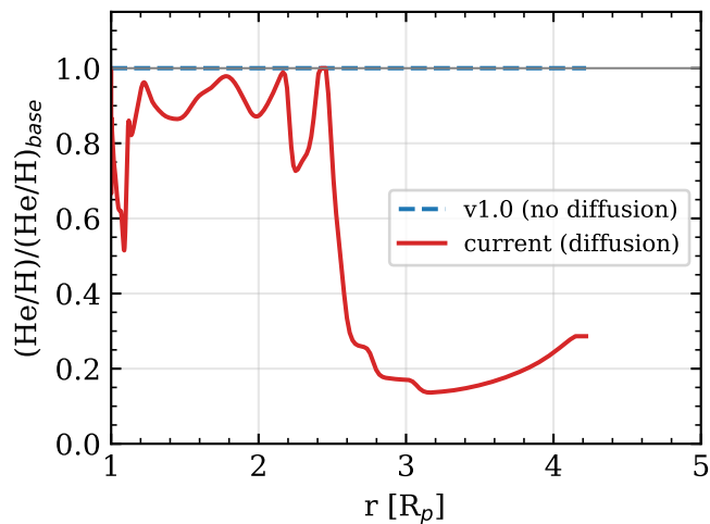
He/H element ratio
