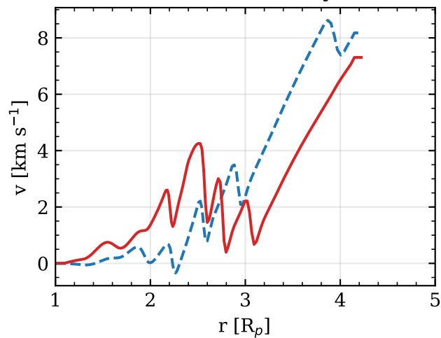
outflow velocity
