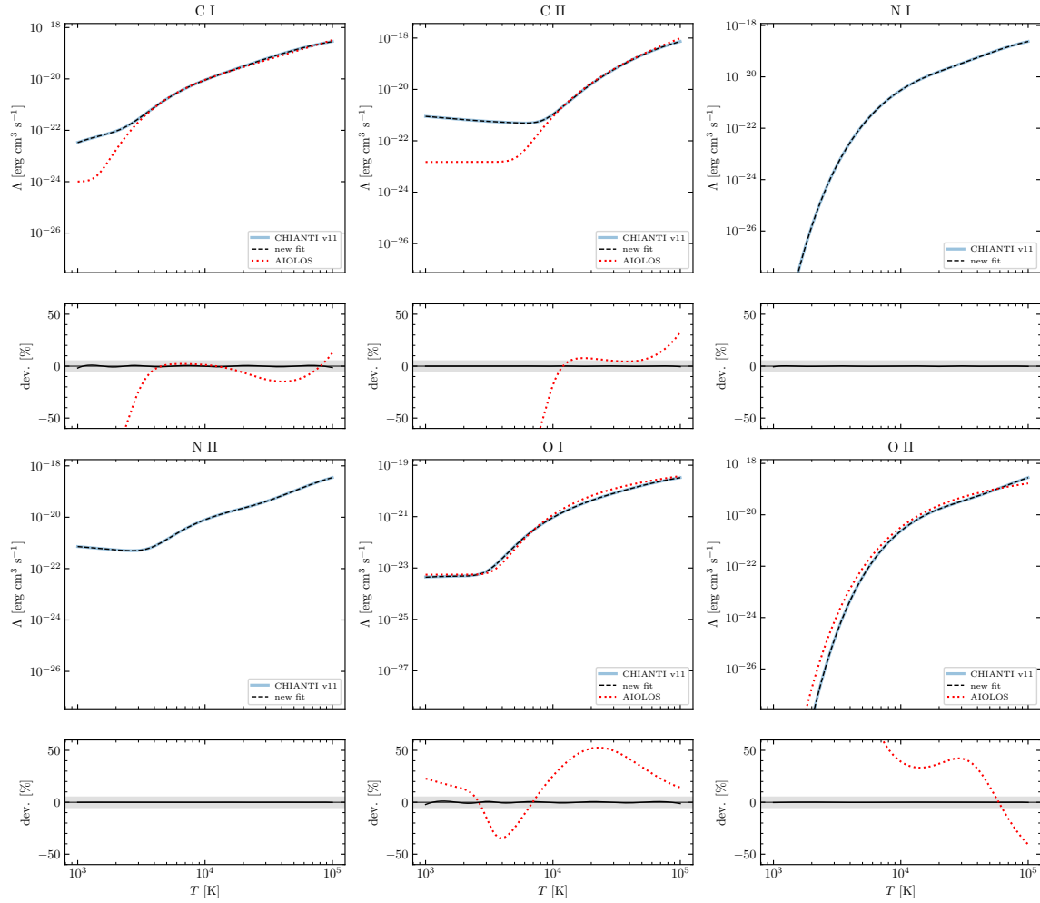
Figure 3: C/N/O line cooling: CHIANTI v11 (solid blue), the new closed-form fits (black dashed), and the AIOLOS formulas (red dotted; absent for nitrogen). Deviation strips show the percentage difference from CHIANTI; the grey band is \pm 5\% .
