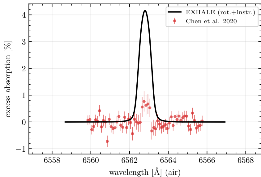
WASP-52 b
