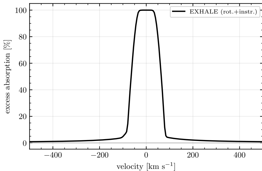
WASP-52 b
