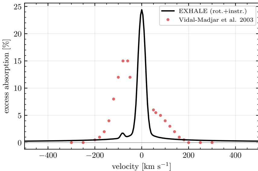
WASP-52 b
