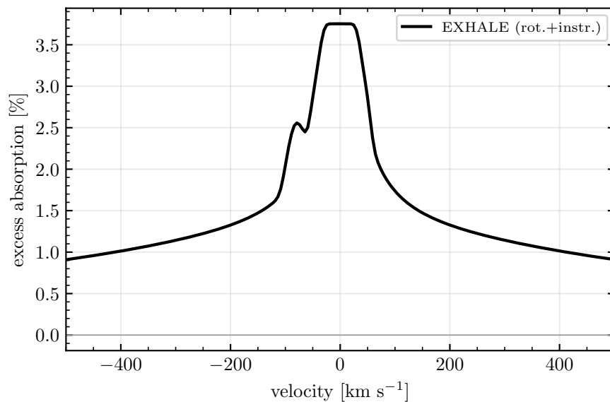
WASP-121 b
