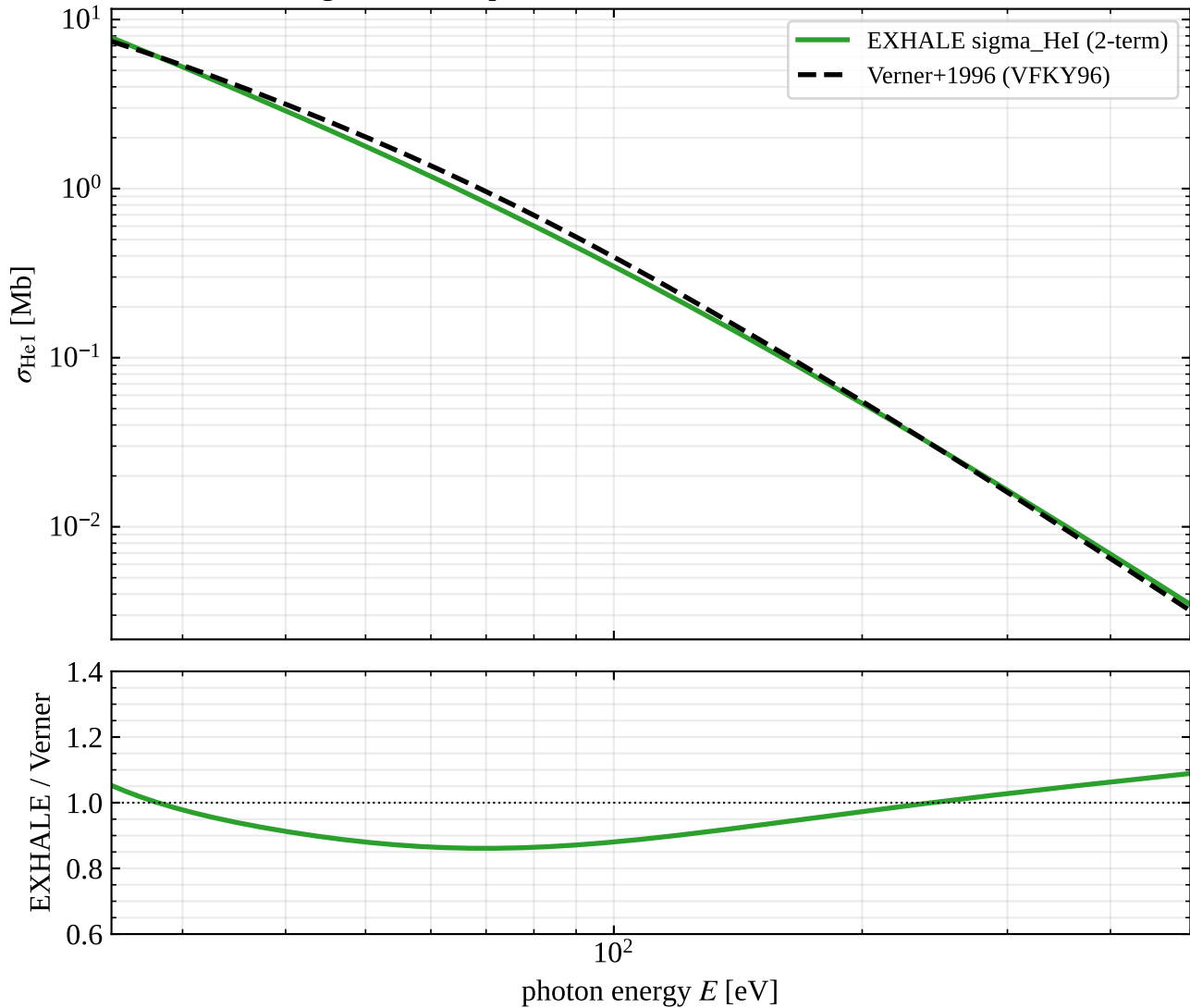
He I ground-state photoionization: EXHALE vs Verner+1996
