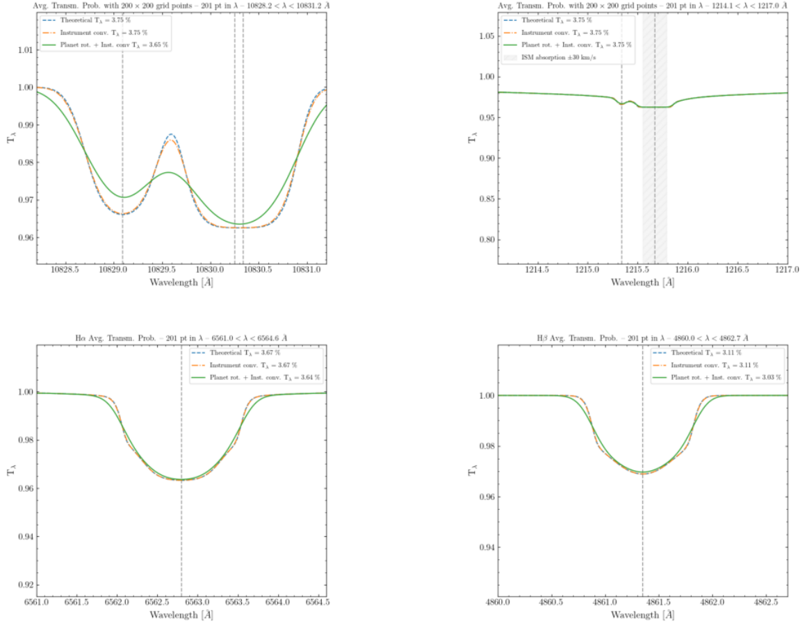
Figure 2: TPM.py output spectra for WASP-121b (Roche, Newton solution with He 2^3 S on; regression/tpm_wasp/ ): He I 10830 (top left), Ly \alpha (top right), H \alpha (bottom left), and H \beta (bottom right). Each panel shows the theoretical line, the instrument-convolved line, and the instrument+rotation-convolved line as produced by the script.
