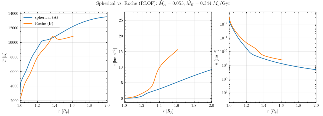
Figure 6: Spherical (Case A) vs. Roche (Case B) WASP-121b: temperature, velocity, and density. The Roche wind reaches L1 ( \approx 1.6R_p ) and accelerates much faster; \dot{M} is annotated. The temperature panel is the _adv profile; its base is smooth because the post-processor falls back to the equilibrium solution where the flow is not a clean outflow (see the caveat in §4.). The Roche velocity (middle) dips slightly negative near the base — the genuine, physical “breathing” inflow of a near-Roche-filling planet.
