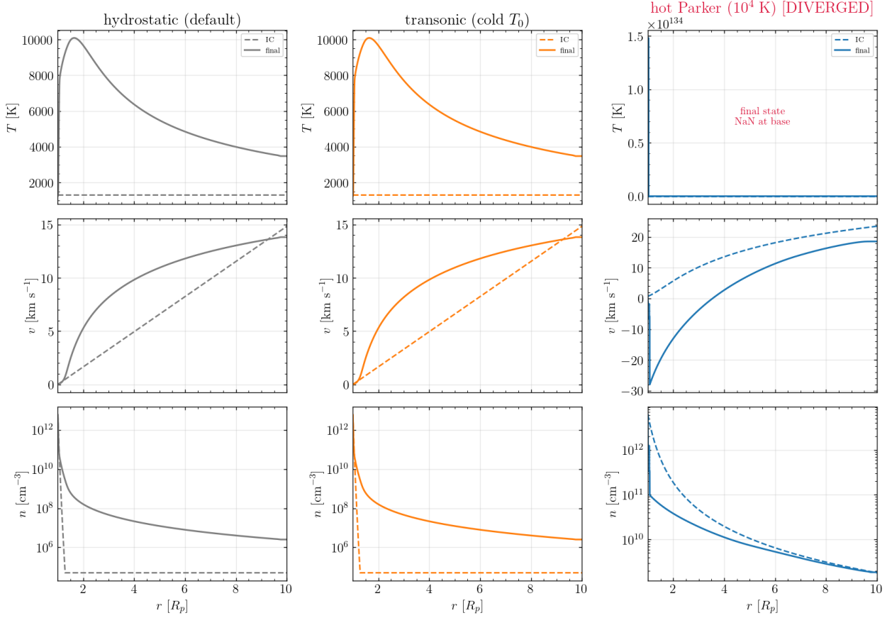
Figure 1: Initial condition (dashed) vs. converged final (solid) for each IC: temperature (top), velocity (middle), density (bottom). hydrostatic and transonic (the latter identical, having fallen back) relax from the flat cold IC to the peaked \sim 10^4 K transonic wind. hot_parker starts from a sane warm-wind IC but its final state diverges (note the 10^{134} K temperature axis and the “NaN at base” annotation; the final velocity turns negative — base inflow).
