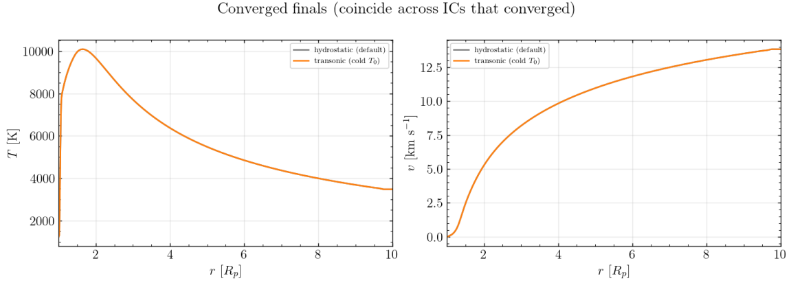
Figure 2: Converged final temperature and velocity for the ICs that converged (hydrostatic and transonic): they coincide, confirming the IC affects only convergence cost, not the steady state. The diverged hot-Parker run is excluded.
