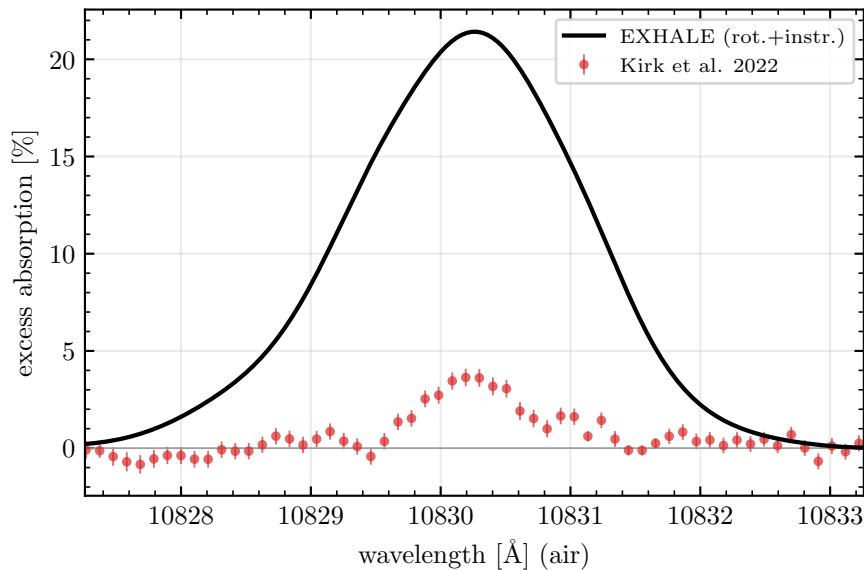
WASP-52 b
