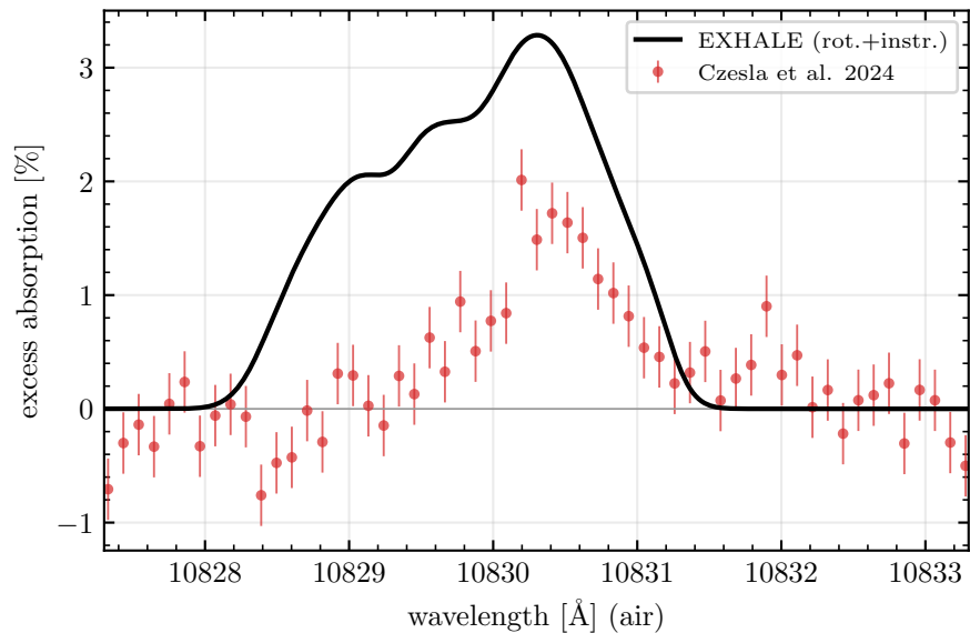
WASP-121 b
