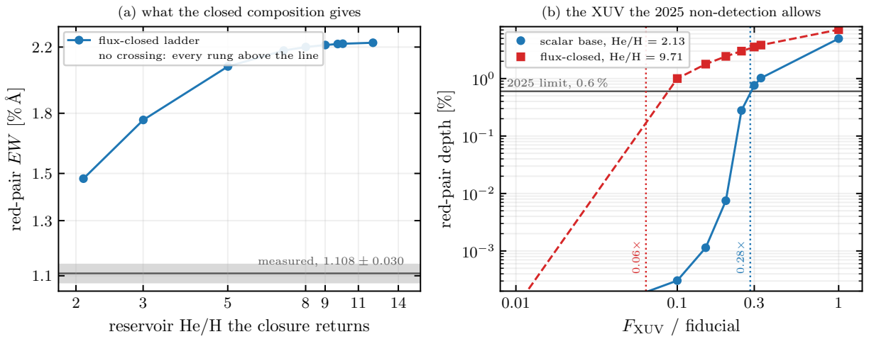
Figure 25: (a) The red-pair equivalent width of the flux-consistent solutions against the reservoir He/H returned (Table 20), with the measured 1.108 \pm 0.030 % Å as the band at the bottom of the panel; every point stands above it, the lowest by 33 per cent, so no crossing is drawn. Every point satisfies the elemental-flux condition, so that condition never picked a reservoir, and on the current code the line does not pick one either. (b) The red-pair depth against the XUV scaling (Table 22), from the scalar base at He/H = 2.13 and the photochemical column at 9.71. The scalar model falls below the 0.6 per cent limit of the 2025 non-detection at about 0.28 of the fiducial irradiation (dotted). The other model is drawn from 0.10 to 1.00, where every point certifies, and continued to its case at 0.01, which does not certify; the 0.06 marked where that last segment crosses the limit is a linear reading between an uncertified point and 0.10, not a measured crossing. On certified states its limit lies below 0.10 and is not bracketed.
