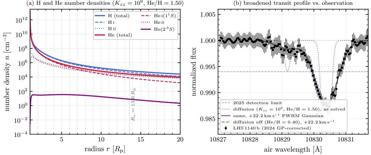
Figure 15: The diffusive solution matched on equivalent width ( \text{He}/\text{H} = 1.50 at K_{zz} = 10^9 \text{ cm}^2 \text{ s}^{-1} ). (a) Absolute number densities of hydrogen species (total H, H I, H II) and helium species (total He, He I( 1^1S ), He II, and metastable He( 2^3S )) as a function of planetary radius r [ R_p ]. At the lower boundary ( r = 1.0 R_p ), \text{He}/\text{H} = 1.50 ; diffusion lets helium settle outward relative to hydrogen, with the local abundance falling to \text{He}/\text{H} = 0.456 at 2 R_p and 0.355 at 10 R_p . Dotted vertical line marks the stellar disk radius ( 13.6 R_p ). (b) The transmission spectrum as solved (dotted purple, its core running below the plotted range) and convolved with the 22.22 \text{ km s}^{-1} FWHM Gaussian that reproduces the measured width (solid purple), against the measurement; the well-mixed curve solved without diffusion, at its own matched Gaussian (dashed green), is repeated from Fig. 12. The two broadened curves are indistinguishable: their Gaussians agree to four digits. All model curves are shifted by the fitted v_{\text{wind}} = +2.26 \text{ km s}^{-1} .
