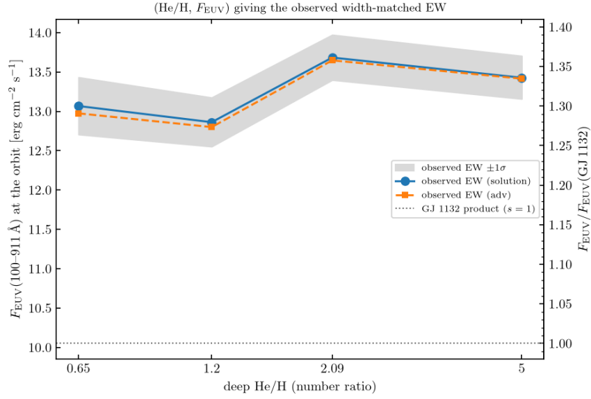
Figure 5: F_{\text{EUV}}(100-911 \text{ \AA}) at the orbit at which the width-matched equivalent width equals the measurement, against the deep He/H: the GJ 1132 spectrum with its flux at \lambda \leq 911.75 \text{ \AA} multiplied by s (bolometric flux held; a sensitivity construction, not a stellar model). Linear interpolation in \ln s between bracketing converged states; solution (circles) and advection-corrected (squares) products; grey band, the 1\sigma of the measurement; dotted, the unscaled GJ 1132 product; right axis, the factor over the GJ 1132 value ( s ). Update log sections 98 and 99.
