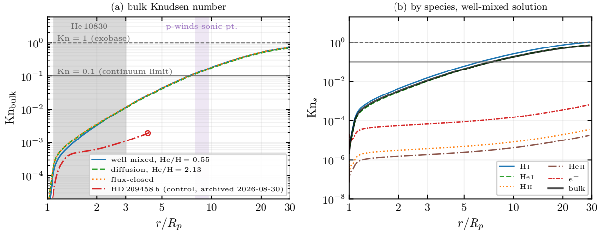
Figure 27: Where the continuum description holds. (a) The bulk Knudsen number of the three representative LHS 1140 b solutions and of the HD 209458 b control, whose sonic point at 4.085 R_p is the open circle; the shaded bands are the He 10830 line-forming region, 1.1\text{--}3 R_p , and the 8\text{--}9.5 R_p at which the p-winds retrieval places its sonic point. The LHS 1140 b solutions cross Kn = 0.1 at 7.30\text{--}7.44 R_p and reach 0.68\text{--}0.71 at the top of the domain, while the control stays below Kn_{\text{bulk}} = 3 \times 10^{-3} everywhere and is collisional through its critical point, over which its largest Kn is 0.018 against 1.00\text{--}1.04 for the LHS 1140 b solutions, a factor of about 55. (b) The species split of the well-mixed solution: neutral hydrogen and neutral helium set the number, while the ions are held by Coulomb collisions four to five orders of magnitude more tightly and the electrons three.
