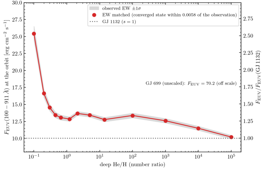
Figure 6: As Fig. 5 for deep He/H = 0.1 to 10^5 (thirteen He/H; solution product; a point is an open circle only if no converged state lies within 0.0058 of the measurement); F_{\text{EUV}}(100\text{--}911 \text{ Å}) at which the width-matched equivalent width equals the measurement; grey band, the 1\sigma of the measurement; dotted, the unscaled GJ 1132 product; right axis, the factor over the GJ 1132 value ( s ). GJ 699 (unscaled) has 70.2, off the scale. Update log sections 102 and 108.
