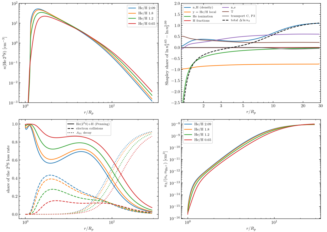
Figure 4: The He(2 3 S) balance of the four states. Top left: n_3 . Top right: Shapley split of \ln n_3^{0.65} - \ln n_3^{2.09} at each radius. Bottom left: share of the 2 3 S loss rate taken by He(2 3 S) + H (solid), electron collisions (dashed) and A 31 (dotted). Bottom right: n_3/(n_e n_{\text{He}^+}) . Source: phase5/dEW_decomposition/fig_n3_balance.png.
