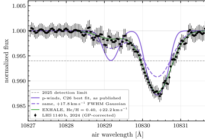
Figure 16: The C26 p-winds best fit as published (solid purple) and convolved with the 17.8 \text{ km s}^{-1} FWHM Gaussian that reproduces the measured width (dashed purple), against the measurement. The EXHALE \text{He}/\text{H} = 0.40 curve at its own matched Gaussian ( 22.2 \text{ km s}^{-1} , thin green) is repeated from Fig. 12. Broadened to the observed width, the p-winds curve passes above the red core, so the width is matched and the depth is not. All curves are shifted by the same v_{\text{wind}} = +2.26 \text{ km s}^{-1} .
