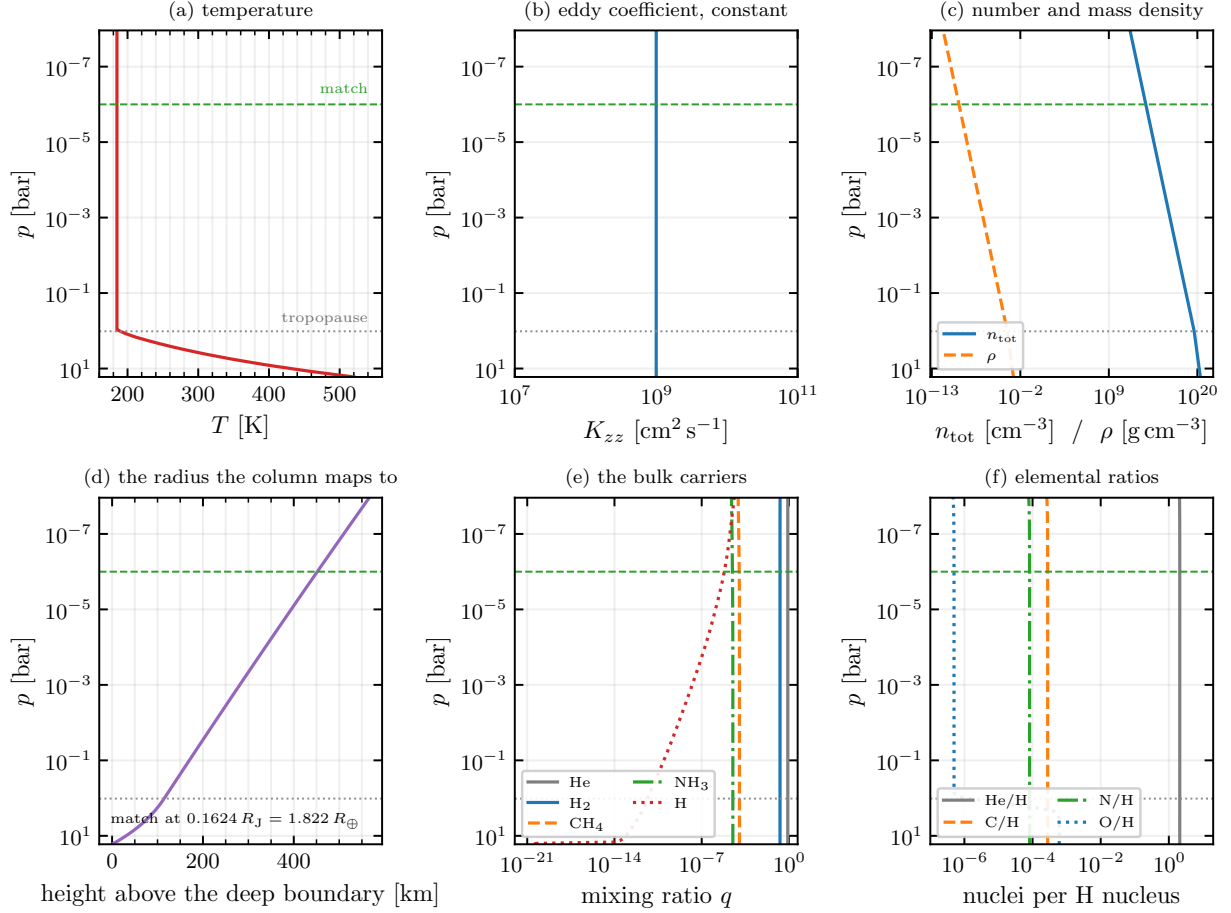
Figure 21: The photochemical column, its structure and the species that carry the bulk of each element. (a) the solved temperature; (b) the eddy coefficient, constant at 10^9 \text{ cm}^2 \text{s}^{-1} over all 102 levels; (c) number and mass density; (d) the radius the pressure grid maps to, which is what fixes the base radius of the wind; (e) the species that hold the bulk: helium reconstructed as \text{He}/\text{H}(2q_{\text{H}_2} + q_{\text{H}}) , and atomic H four to five decades below \text{H}_2 everywhere; (f) the elemental ratios the profile hands over. The tropopause (1.031 bar, dotted) and the 1 \mu bar matching level (dashed) are marked on every panel. Fig. 26b,c shows the same climate and elemental ratios in the context of the iteration, while this figure shows the file itself, column by column.
