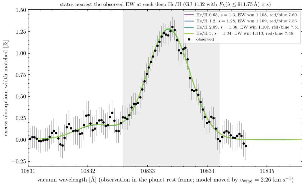
Figure 7: Width-matched excess absorption of the converged state nearest the measured equivalent width at each deep He/H (route B, steps 2 and 3), over the observed spectrum (vacuum wavelength, planet rest frame; grey band, the equivalent-width window). The model curves are moved by the fitted v_{\text{wind}} = +2.26 \text{ km s}^{-1} for the overlay only, as in the earlier figures; every equivalent width and metric is from the unshifted spectra. The kernel FWHM f is chosen for each curve to reproduce the observed FWHM; it stands for a velocity field the one-dimensional model does not contain.
