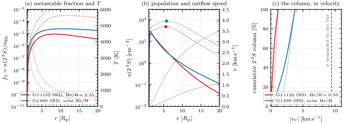
Figure 17: The adiabatic-cooling metastable bump in the EXHALE solutions (solid: advection-corrected, the profiles the transit integral uses; dotted: local equilibrium; faint curves on the right-hand axes). Two cases of Table 12 are drawn: He/H = 0.55 on the GJ 1132 proxy and solar He/H on the GJ 699 one. (a) The metastable fraction rises outward over the cooling leg, from the temperature maximum out to a maximum of f_3 at 11.6 and 11.8 R_p in equilibrium, which is the bump in the sense of Schulik & Owen (2025). (b) The equilibrium n_{2^3S} peaks at 5.6–5.7 R_p (markers); advection moves the maximum inward, to 1.4–1.5 R_p , and quenches the outer rise. (c) The absorber-weighted distribution of |v_r| over the 2^3S column: the whole column lies below 4 \text{km s}^{-1} , far short of the \sigma = 9.4 \text{ km s}^{-1} the measured width demands.
