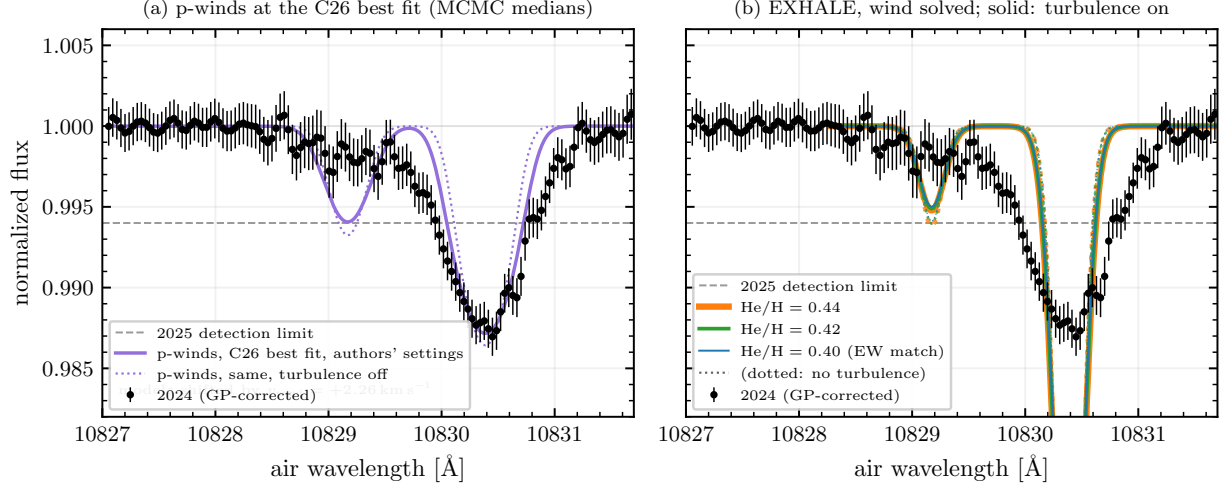
Figure 8: The measurement is in black. On the left is the paper’s own p-winds model at its best fit, the MCMC medians its Fig. 4 legend states, computed with the authors’ released settings; that model is the solid curve and the dotted one is the same run with turbulence off. On the right is EXHALE at the three well-mixed compositions of record that bracket the equivalent-width crossing 0.4044: \text{He}/\text{H} = 0.40 , the solved case nearest the crossing, with 0.42 and 0.44. For each of them a second spectrum was synthesized on the same solution with the turbulence term on, so the solid EXHALE curves carry the same turbulence term p-winds uses and the dotted ones are without it. Over that range of composition the profile barely moves, so the three nearly coincide; the composition dependence of the absorbing power is Fig. 11. Neither code applies a line-of-sight bulk velocity, so both sets of model curves are shifted by the v_{\text{wind}} = +2.26 \text{ km s}^{-1} that C26 fit. The shift is applied to the plotted curves only: every equivalent width in this memo is computed on the unshifted spectra, the observation in the planetary rest frame of its released file. The figure is drawn in the presentation of the paper’s Fig. 4.
