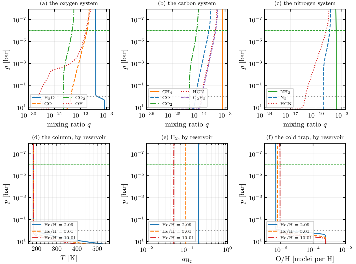
Figure 22: The molecular systems, and what the reservoir does to them. (a)–(c) the oxygen, carbon and nitrogen species of the same file: water condenses out at the tropopause while \text{CH}_4 and \text{NH}_3 cross it unchanged, and the photochemical products ( \text{HCN} , \text{C}_2\text{H}_2 , \text{N}_2 , \text{CO} , \text{OH} ) climb several decades in the top of the column while staying trace. (d)–(f) the same column solved at three reservoirs of the earlier sequence: the deep boundary cools as helium is added, \text{H}_2 is diluted by number, and the cold trap loosens, so oxygen is the one element the reservoir moves. Levels are marked as in Fig. 21.
