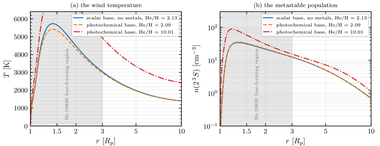
Figure 24: The thermostat, on the three solutions of Table 19. (a) temperature and (b) the metastable density, against radius, with the He 10830 line-forming region 1\text{--}3R_p shaded. Adding the photochemical column's C, N and O at fixed reservoir (solid to dashed) now costs the wind 315 K in T_{\text{max}} and leaves the metastable population where it was, to within 2 per cent in the peak and in the column. Raising the reservoir on that same base (dashed to dot-dashed) reheats it by 2267 K and lifts the metastable peak by 2.5.
