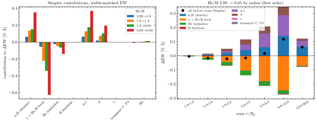
Figure 3: Left: Shapley contributions of the nine factor fields to the change of the width-matched equivalent width, for the three adjacent pairs and for 2.09 \rightarrow 0.65 . Right: 2.09 \rightarrow 0.65 split by radial zone, first order for each factor (bars), with the zone Shapley value of all factors together (diamonds). Source: phase5/dEW_decomposition/fig_dEW_factors.png.
