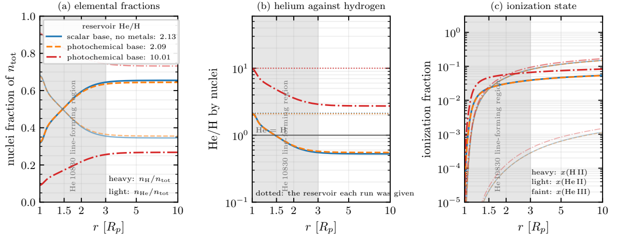
Figure 23: Composition and ionization against radius, for the three solutions of Table 19, from the same advection-corrected profiles. (a) the hydrogen and helium nuclei fractions of n_{\text{tot}} ; (b) He/H by nuclei, with the reservoir each run was given as a dotted line, so the vertical drop from dotted line to curve is what element diffusion does; (c) the ionization fractions. n_{\text{tot}} counts one particle per species, H I, H II, He I, He II, He III and every metal ion stage, with electrons excluded, and He 2^3S not added because it is an excited level inside He I, so (a) does not sum to one on the photochemical base. The metals it misses are negligible: their largest share of n_{\text{tot}} anywhere in 1\text{--}30R_p is 2.3 \times 10^{-4} at He/H = 2.09 and 9.7 \times 10^{-5} at 10.01, and zero on the metal-free base. Nuclei are counted as H I + H II and He I + He II + He III. The flux-consistent sequence does not cross the measurement anywhere (Sect. 15.7), so no crossing is marked between the two profile runs drawn here. The He 10830 line-forming region 1\text{--}3R_p is shaded.
