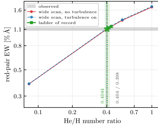
Figure 11: Red-pair equivalent width against composition, with and without the turbulence term, compared with the measured band. The crossing is insensitive to the broadening treatment: each solved composition of the well-mixed group up to \text{He}/\text{H} = 1 carries both syntheses of the same solution, so the two curves differ only in the broadening, and they cross the measured band at \text{He}/\text{H} = 0.4044 without the turbulence term and 0.3985 with it, 1.5 per cent apart. The three compositions 0.40 , 0.42 and 0.44 drawn on top are where the spacing brackets the measurement directly.
