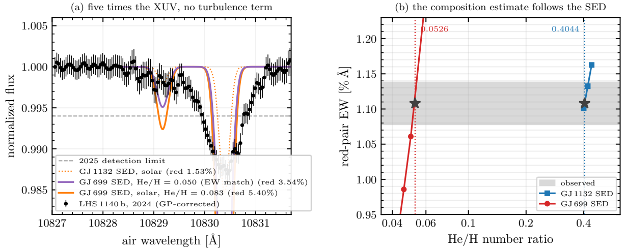
Figure 20: The GJ 699 proxy, five times the XUV of the GJ 1132 proxy used elsewhere in this memo. Left: the measurement with the EXHALE solution nearest the equivalent-width crossing 0.0526, the one at \text{He}/\text{H} = 0.050 , and the solar case on this spectrum, with the GJ 1132 solar case dotted for contrast; all curves without the turbulence term and shifted by the fitted v_{\text{wind}} = +2.26 \text{ km s}^{-1} . The lines are deeper but no wider, the GJ 699 solar curve reaching 3.5\times the depth of the GJ 1132 one (5.40% against 1.53%) while the added broadening the measurement demands of the two differs by 0.45 \text{ km s}^{-1} , or 2 per cent (21.95 against 22.40 \text{ km s}^{-1} ). Right: red-pair equivalent width against composition for the two spectra, with the measured band and the two crossings; the composition the line implies moves from 0.4044 to 0.0526 when the assumed spectrum is changed.
