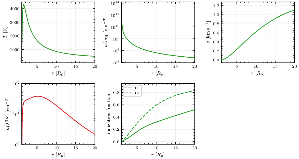
Figure 19: The EXHALE solution matched on equivalent width (the solved composition \text{He}/\text{H} = 0.40 , nearest the well-mixed crossing at 0.4044): temperature, density, velocity, metastable helium density, and ionization fractions. Dotted vertical line: the stellar radius.
