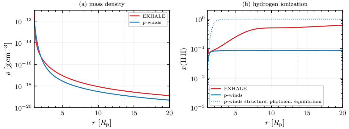
Figure 10: The other two profiles of the same comparison ( \text{H}:\text{He} = 10^{-3} , same spectrum): (a) mass density, (b) hydrogen ionization. The dotted curve in (b) is photoionization equilibrium evaluated on p-winds' own density and temperature, so its distance from the solid p-winds curve is how far the imposed flow holds hydrogen out of equilibrium. Dotted vertical line: the stellar radius.
