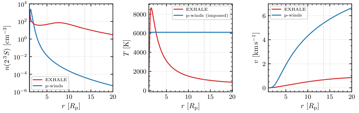
Figure 9: Same composition ( \text{H}:\text{He} = 10^{-3} ), same spectrum, two wind structures. Dotted vertical line: the stellar radius, 13.6R_p .
