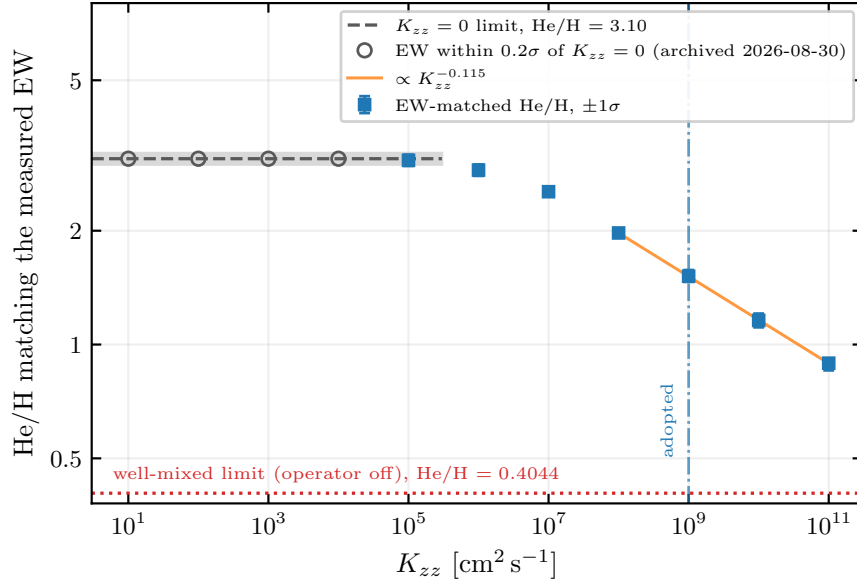
Figure 13: The composition–mixing degeneracy in full. Each square is the He/H reservoir ratio whose red-pair equivalent width equals the measured one, solved at one decade of K_{zz} with helium and hydrogen free to separate by diffusion (Table 9); the error bars propagate the measurement error alone and are smaller than the symbols over most of the range. The landscape has three parts. Below K_{zz} \simeq 10^5 the eddy term is a small correction to the molecular coefficient the base already carries, the inference sits on a plateau at He/H = 3.10 (dashed, with its 1\sigma band), and the open circles mark the decades whose equivalent width, on the 2026-08-30 solutions, differed from the K_{zz} = 0 one by less than a fifth of the measurement error. Between 10^6 and 10^7 the curve rolls off. From 10^8 up it is the shallow power law K_{zz}^{-0.115} (orange, fitted to those four points). Neither end of the axis reaches the well-mixed crossing of 0.4044 (dotted): with diffusion active, helium settles at every eddy coefficient tried, and He/H inferred from this line is a statement about the assumed mixing as much as about the planet. The adopted K_{zz} = 10^9 \text{ cm}^2 \text{ s}^{-1} is marked.
