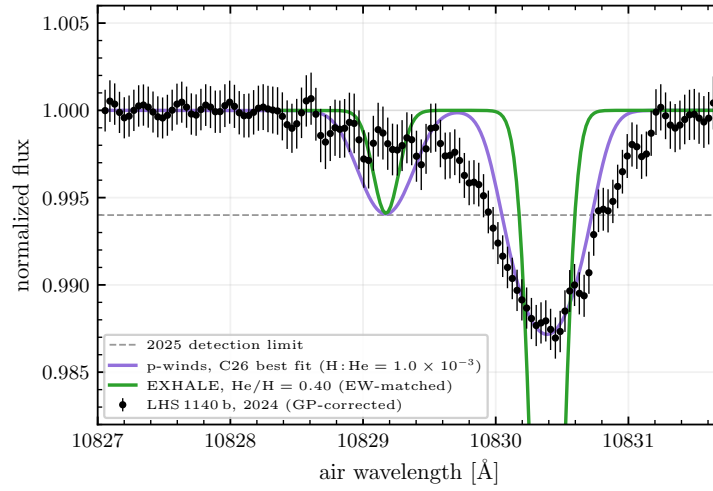
Figure 18: The two best models over the 2024 spectrum, in the presentation of the paper’s Fig. 4: p-winds at the C26 best fit (the MCMC medians) with the authors’ settings, and EXHALE at the composition matched on equivalent width, \text{He}/\text{H} = 0.40 . Both are shifted by the fitted v_{\text{wind}} = +2.26 \text{ km s}^{-1} .
