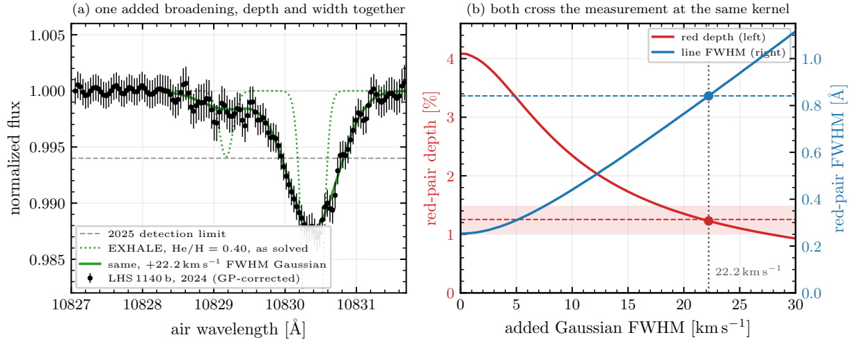
Figure 12: Left: the EXHALE profile matched on equivalent width as solved (dotted, its core running below the plotted range) and convolved with a 22.22 \text{ km s}^{-1} FWHM Gaussian (solid), against the measurement. Both are shifted by the same v_{\text{wind}} = +2.26 \text{ km s}^{-1} used in the earlier figures. Right: red-pair depth (red, left axis) and red-pair FWHM (blue, right axis) as the added Gaussian is scanned. Dashed lines are the observed values, the shaded band the C26 1\sigma interval on the depth; the dotted vertical marks where the width is matched. Both curves meet the measurement at the same Gaussian.
