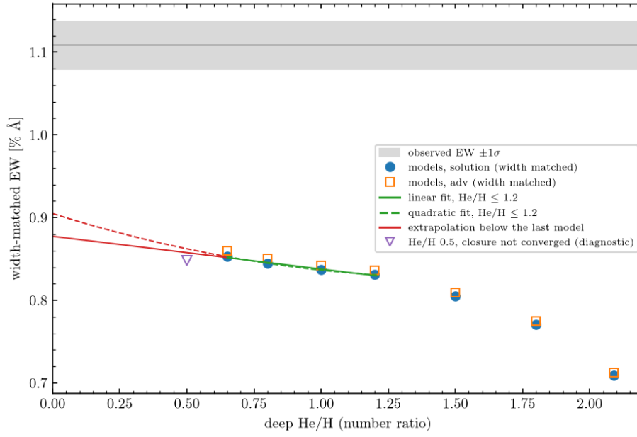
Figure 1: Width-matched equivalent width against the deep He/H, solution (filled) and advection-corrected (open) products, with the linear and quadratic fits over \text{He}/\text{H} \leq 1.2 and their continuation to \text{He}/\text{H} = 0 (extrapolation, red). The triangle is the unconverged \text{He}/\text{H} = 0.5 closure. Grey band: the observed equivalent width and its 1\sigma interval. Source: phase5/fig_ew_vs_heh.png.
