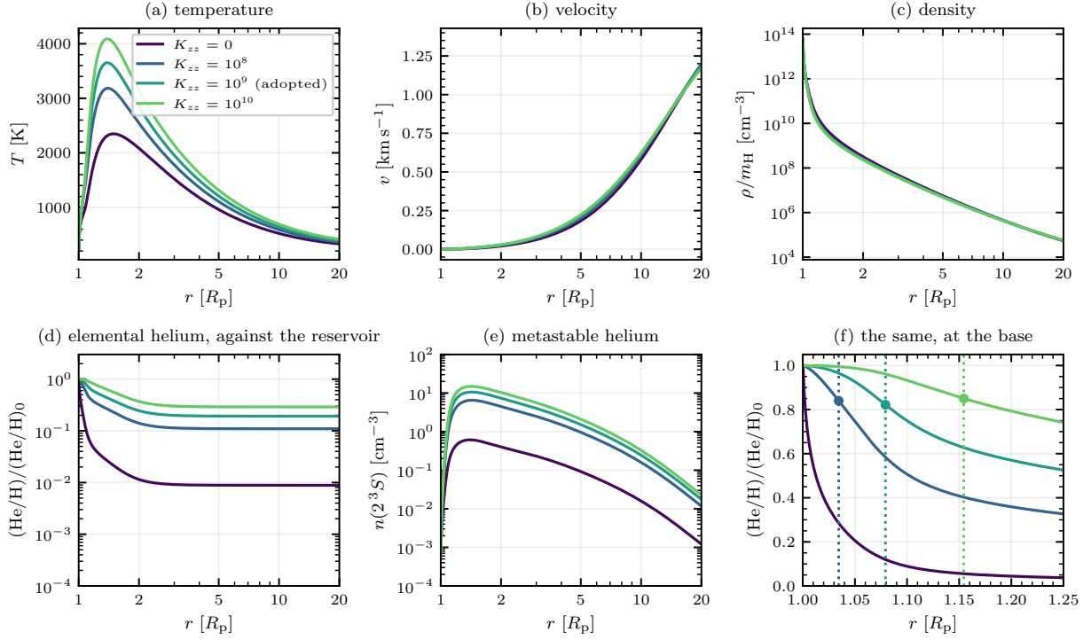
Figure 14: Four solutions differing only in the eddy coefficient, at a fixed reservoir \text{He}/\text{H} = 0.55 with helium and hydrogen free to separate by diffusion: K_{zz} = 0, 10^8, 10^9 (adopted) and 10^{10} \text{ cm}^2 \text{ s}^{-1} , dark to light. The eddy coefficient acts on the composition, not on the wind. Panels (d)–(f), the elemental helium against its base reservoir value and the metastable population: at 1.05 R_p the elemental ratio is 0.206, 0.745, 0.927 and 0.988 of the reservoir and at 5 R_p it is 0.009, 0.110, 0.193 and 0.291, while the peak n(2^3S) is 0.61, 6.5, 10.6 and 14.9 \text{ cm}^{-3} . In panels (b) and (c) the velocity at 10 R_p moves by 8% and the density at 2 R_p by 28%, and \log_{10} \dot{M} by 0.02 dex. Panel (a) is the exception: T at 1.5 R_p rises from 2349 to 4006 K, because the helium the eddy term lifts is itself absorbing. Panel (f) repeats (d) on a linear axis over the base, where the dots and dotted lines mark each run’s homopause, the radius at which its own molecular coefficient equals its K_{zz} , at 1.034, 1.079 and 1.154 R_p , with the K_{zz} = 0 homopause below the base. The table of fluxes through the cell faces that the homopause is read from is written only when the run is asked for it, and comes from these same four solutions post-processed a second time with that output turned on.
