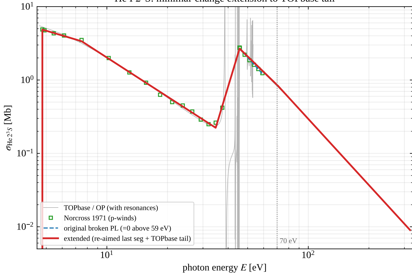
He I 2^3S : minimal-change extension to TOPbase tail
