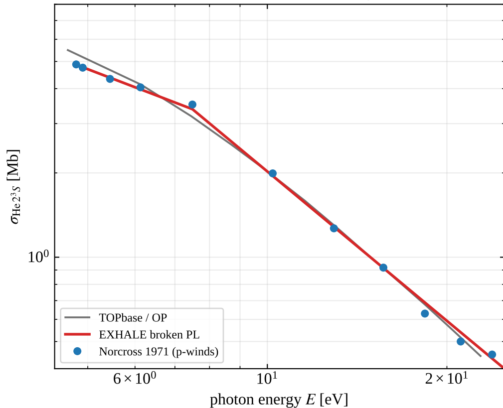
(b) Smooth near-threshold region
