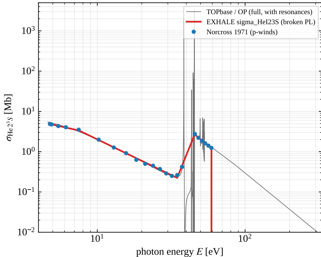
(a) Full range: TOPbase resonance structure
