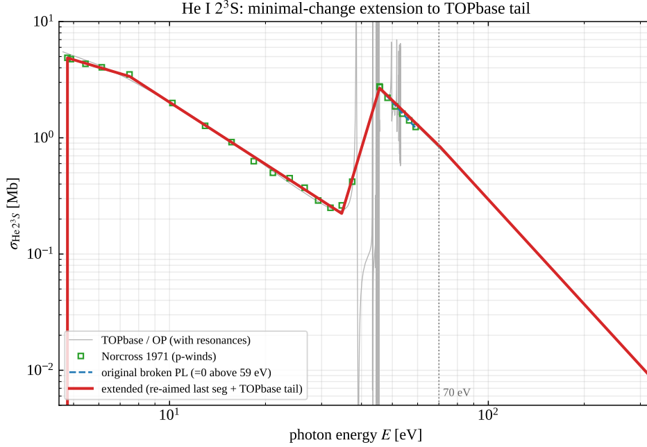
Figure 7: Recommended minimal-change extension (red): the original broken power law up to the 45.6 eV bump, a re-aimed last segment (slope -3.039 \rightarrow -2.658 ) reaching the TOPbase fit at 70 eV (dotted line), and the TOPbase power-law tail above. Norcross/p-winds (green) and TOPbase (gray) are overplotted; the original broken power law (blue dashed) cuts to zero at 59 eV. The curve is continuous at both joins.
