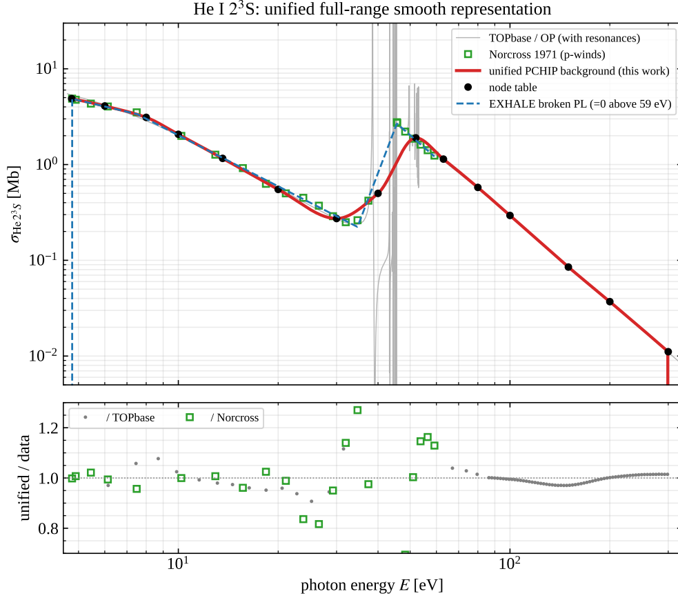
Figure 6: Unified full-range representation (red) of \sigma_{\text{He } 2^3\text{S}} : log–log PCHIP through the node table (black points; Table 7) following the TOPbase resonance-averaged background (gray, with resonances). The Norcross (1971) / p-winds table (green squares) and the current EXHALE broken power law (blue dashed; cut to zero above 59 eV) are overplotted. Bottom: ratio of the unified fit to the TOPbase smooth-background points (gray) and to the Norcross points (green); both within \sim \pm 15\% , with the larger Norcross scatter at 40–55 eV reflecting its coarse sampling of the resonance region.
