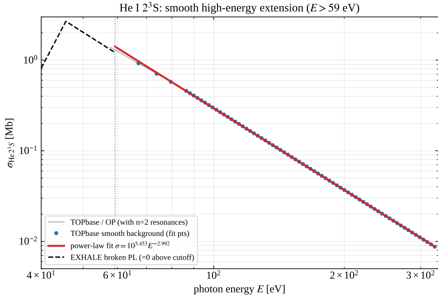
Figure 5: Smooth high-energy extension of \sigma_{\text{He I } 2^3\text{S}} . The power-law fit (red) to the resonance-free TOPbase background (blue points, E \geq 66 eV) follows \sigma \propto E^{-2.99} to \sim 5\% up to 320 eV. The current EXHALE broken power law (black dashed) rises to a resonance-averaged bump near 45 eV and is cut to zero above 59.2 eV (dotted line).
