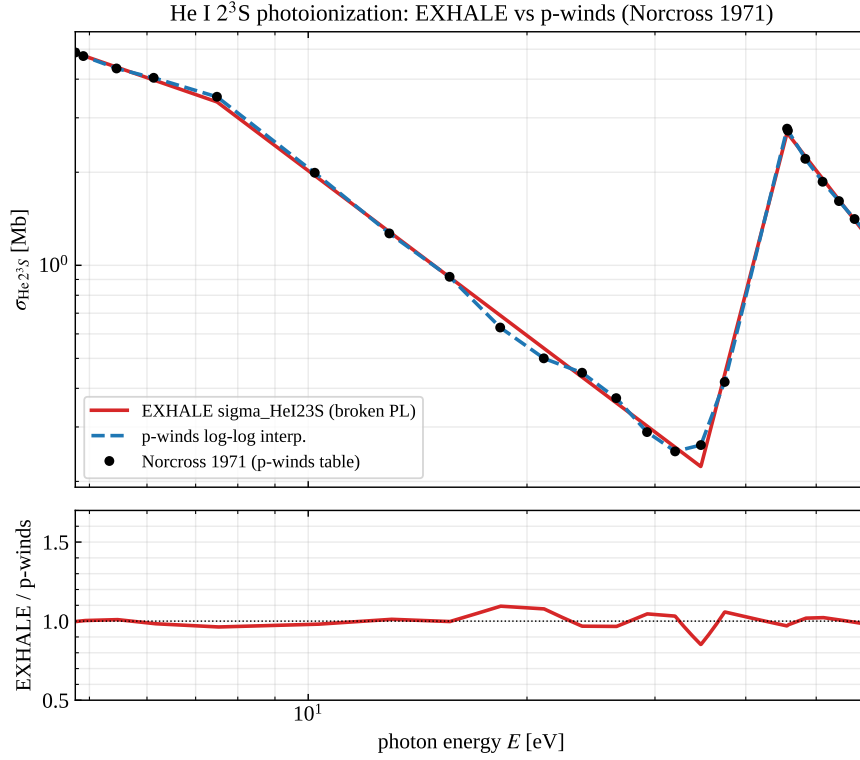
Figure 3: He I 2 3 S photoionization cross section: EXHALE broken power law (sigma_HeI23S, red) vs the p-winds log–log interpolation (blue dashed) of the Norcross (1971) table (black points). Bottom panel: ratio EXHALE/p-winds.
