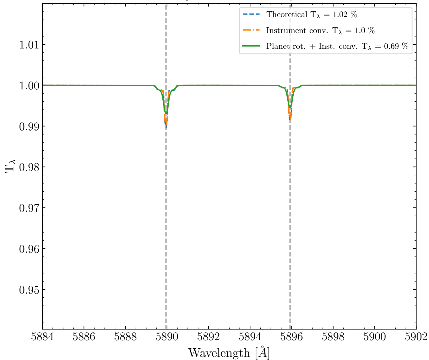
Na I D Avg. Transm. Prob. – 541 pt in \lambda
