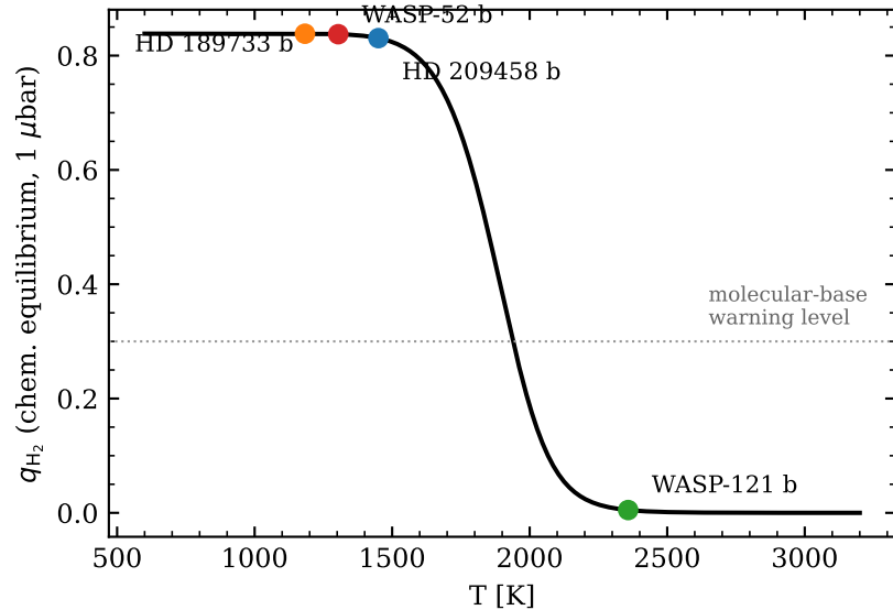
(a) equilibrium \text{H}_2 fraction at the base
