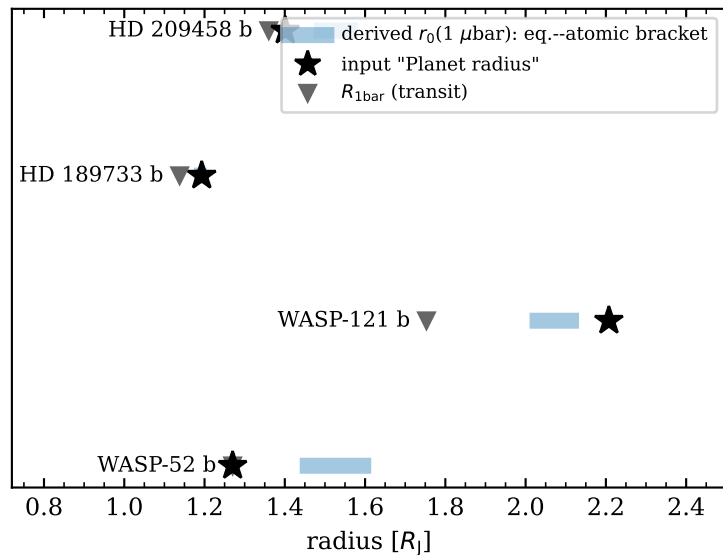
(b) base-radius consistency check
