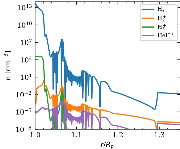
(c) HD 209458 b: molecular species
