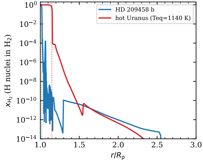
(a) \text{H}_2 \rightarrow \text{H} dissociation fronts
