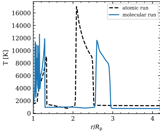
(b) HD 209458 b: T (3000-step relaxation snapshot)
