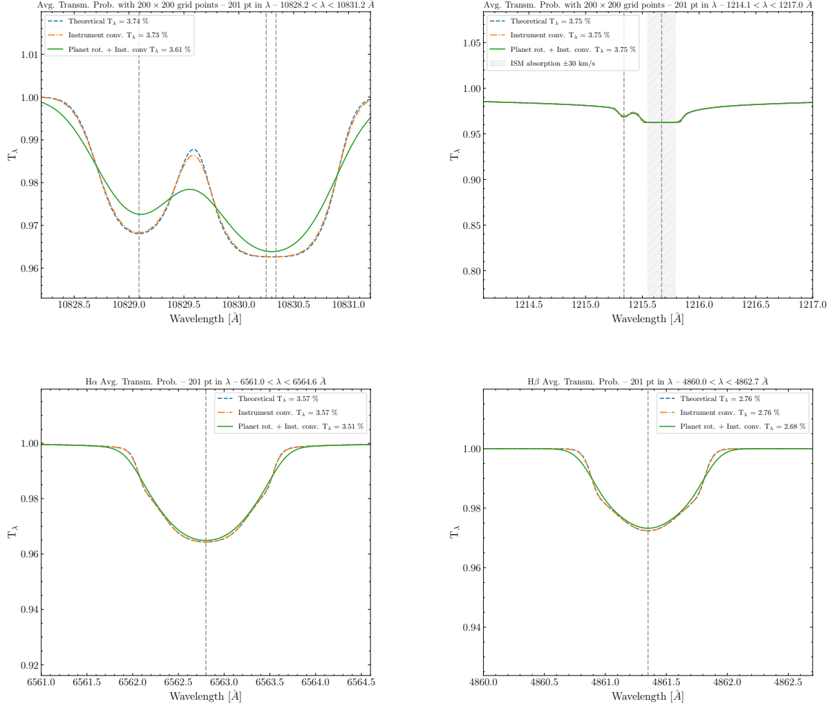
Figure 2: EXHALE_transit.py output spectra for WASP-121b (Roche, Newton solution with He 2 3 S on; backup/regression/tpm_wasp/ ): He I 10830 (top left), Ly \alpha (top right), H \alpha (bottom left), and H \beta (bottom right). Each panel shows the theoretical line, the instrument-convolved line, and the instrument+rotation-convolved line as produced by the script.
