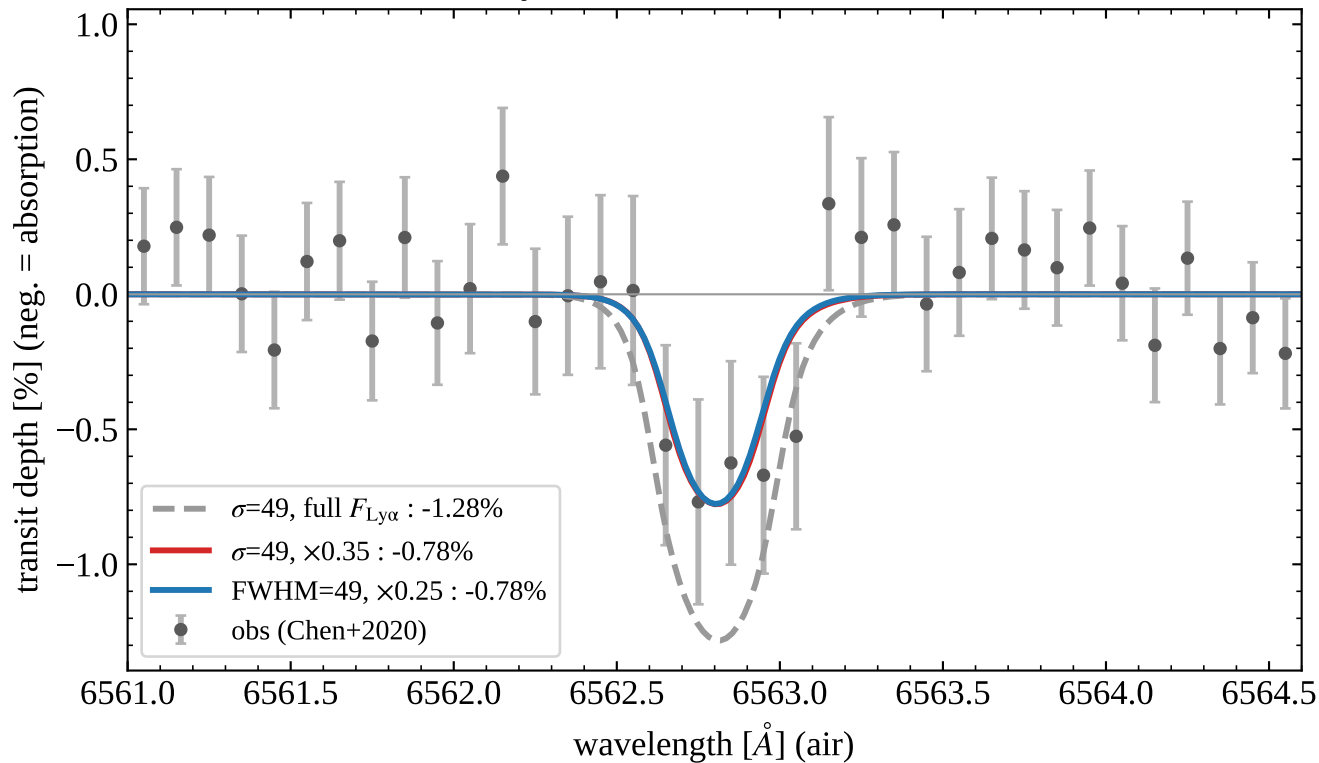
H \alpha : Ly \alpha flux scaled to match the data
