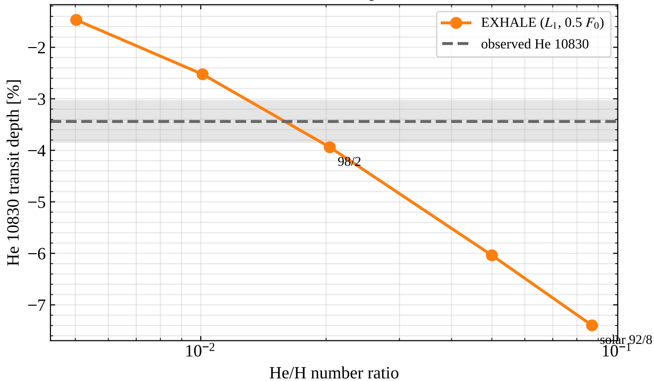
He 10830 vs composition
