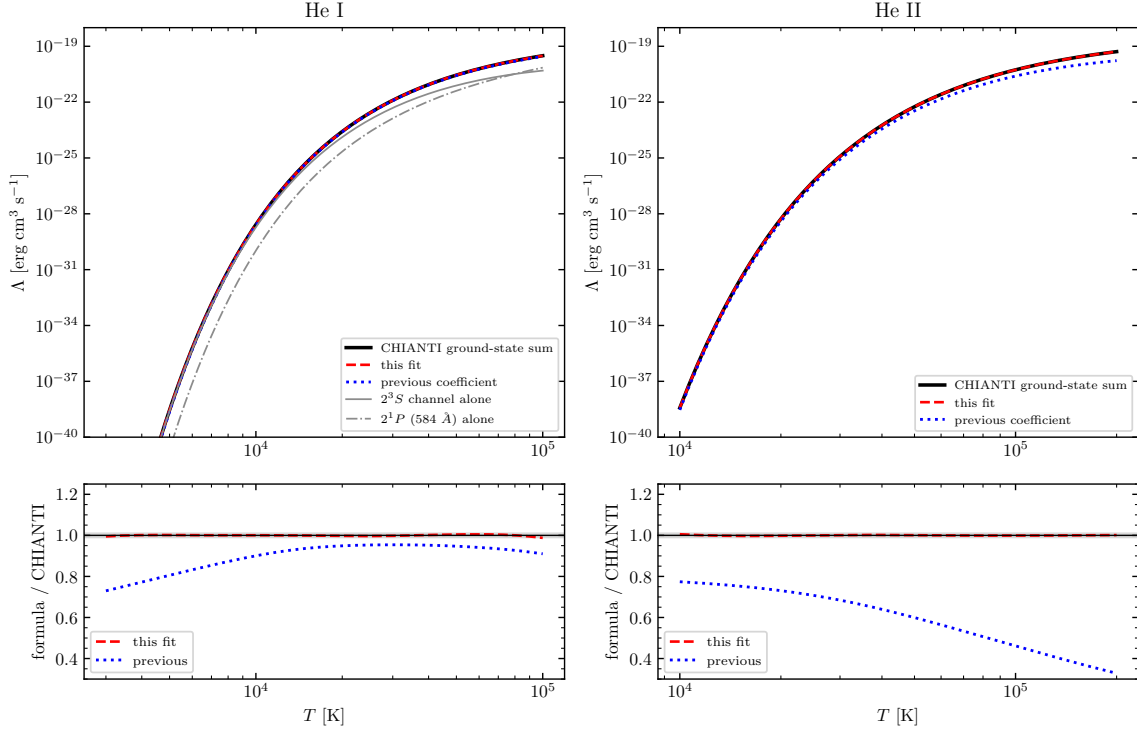
Figure 2: Helium ground-state collisional-excitation cooling: CHIANTI sum (solid black), the fits of Table 2 (red dashed) and the expressions still in the code (blue dotted). For He I the two individual channels most often named are shown in grey: the metastable 2^3S channel that sets the exponent, and the 584 Å resonance line, which stays well below the total at wind temperatures. Bottom: ratio to the CHIANTI sum, with a \pm 1\% grey band.
