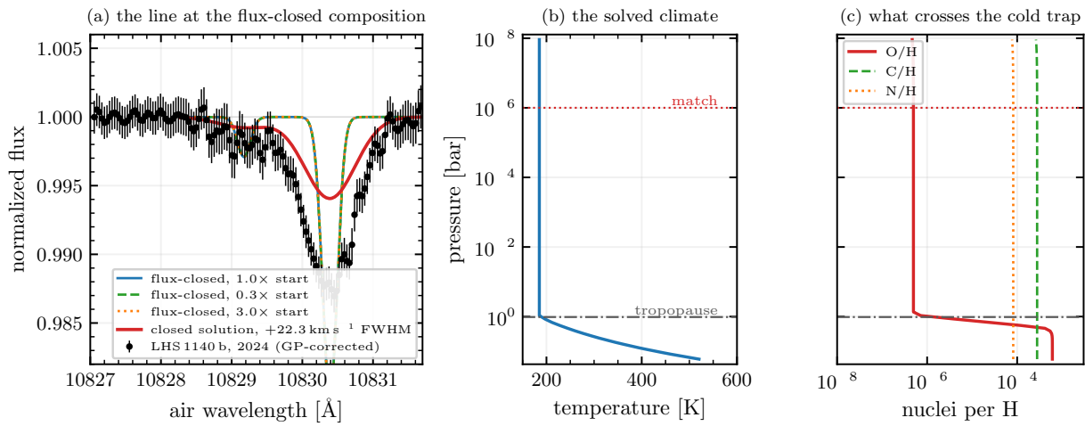
Figure 19: The flux-closed solution and the column it stands on. (a) The three closure arms (started a factor of ten apart in the trial escape flux) are indistinguishable, and all three fall well short of the measured line in absorbing power; the thick curve is the reference arm convolved with the 22.3 \text{ km s}^{-1} FWHM Gaussian that reproduces the observed width, which then lands below the observed depth because the equivalent width was already short. Model curves are shifted by the fitted v_{\text{wind}} = +2.26 \text{ km s}^{-1} , as elsewhere in this memo. (b) The solved climate of the column handed over, with the tropopause at 1.031 \text{ bar} and the 1 \mu\text{bar} matching level marked; the stratosphere sits at the skin temperature, 185 \text{ K} . (c) The elemental abundances the profile carries. Oxygen is cut by a factor 1223 at the tropopause by the water cold trap, while carbon and nitrogen cross it unchanged, and it is those two, not the helium, that make this solution's line 2.6\times weaker than the metal-free base at the same reservoir (Sect. 11.6; both sides of that factor are re-measured on the current binary, and it has now survived both corrections to the physics). Panels (b) and (c) place the column in the closure; the file itself, every column of it, is Figs. 14 and 15.
