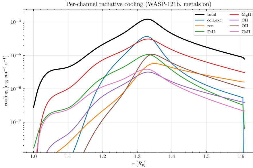
Figure 5: Per-channel radiative cooling vs. radius (WASP-121b, metals on; from Cooling_breakdown.txt). Below \sim 1.4 R_p the metal lines (e.g. Fe II, Mg II, C/O) compete with or dominate the H/He collisional channels.
