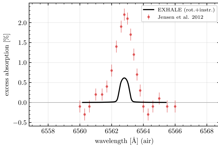
WASP-121 b
