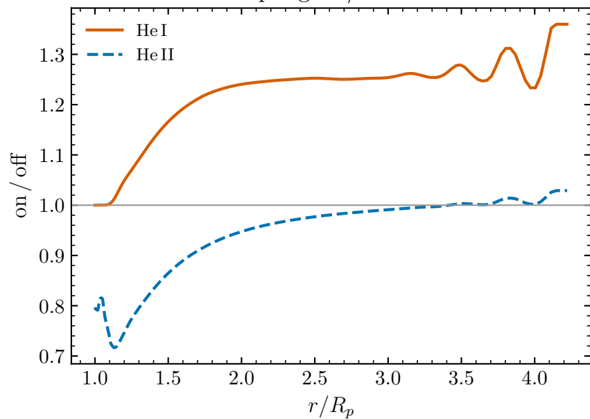
Photoheating rate
