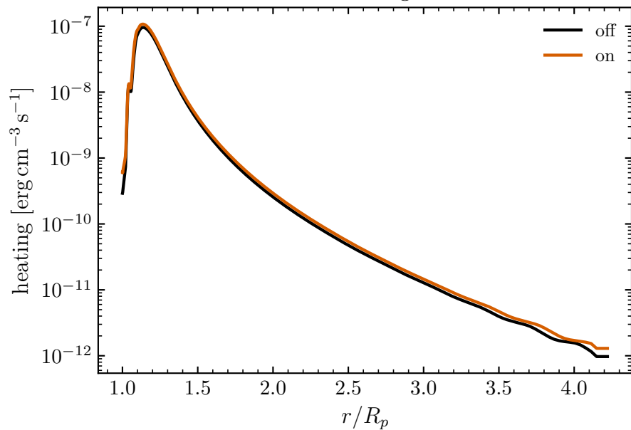
Photoheating rate
