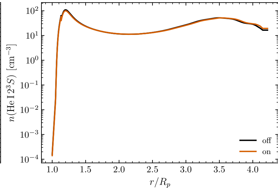
Metastable 2^3S density
