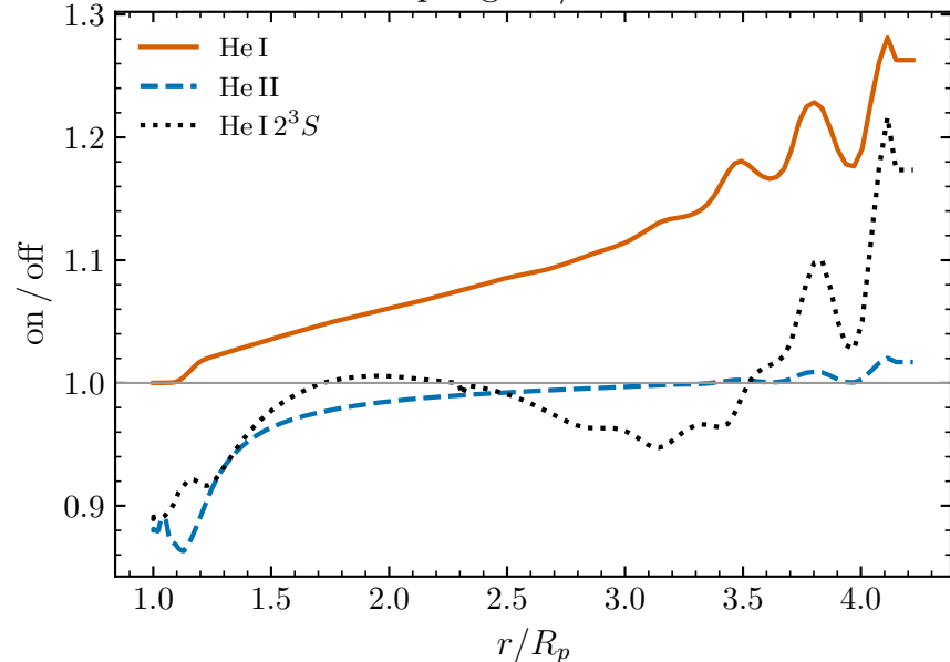
Metastable 2^3S density
