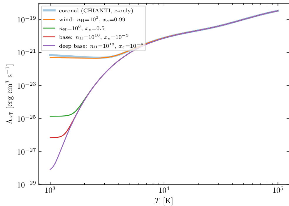
N II
