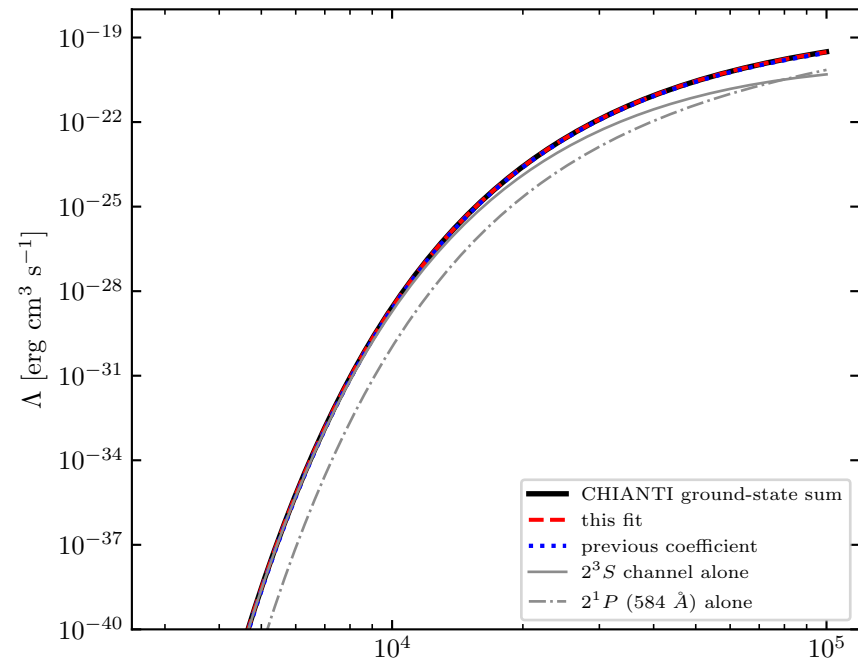
He I
