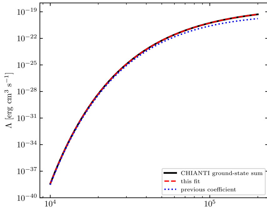
He II
