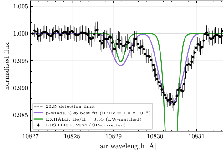
Figure 6: The two best models over the 2024 spectrum, in the presentation of the paper’s Fig. 4: p-winds at the C26 best fit (the MCMC medians) with the authors’ settings, and EXHALE at the equivalent-width-matched composition. Both are shifted by the fitted v_{\text{wind}} = +2.26 \text{ km s}^{-1} .
