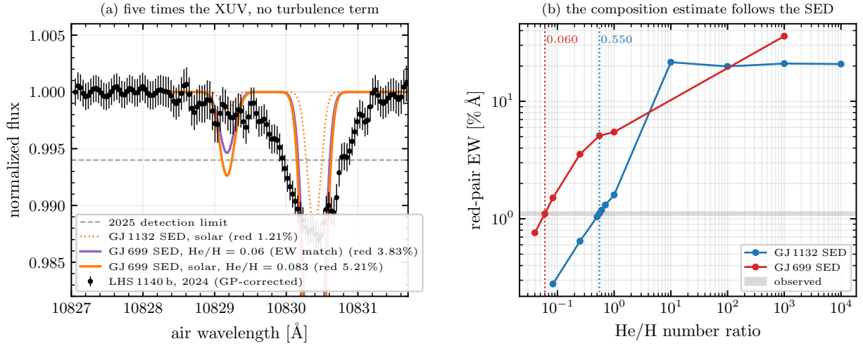
Figure 8: The GJ 699 proxy, five times the XUV of the GJ 1132 proxy used elsewhere in this memo. Left: the measurement with the EXHALE solution nearest the equivalent-width crossing ( \text{He}/\text{H} = 0.06 ) and the solar case on this spectrum, with the GJ 1132 solar case dotted for contrast; all curves without the turbulence term and shifted by the fitted v_{\text{wind}} = +2.26 \text{ km s}^{-1} . The lines are deeper and no wider. Right: red-pair equivalent width against composition for the two spectra with the measured band and the two crossings; the composition the line implies moves from 0.550 to 0.060 when the assumed SED is changed.
