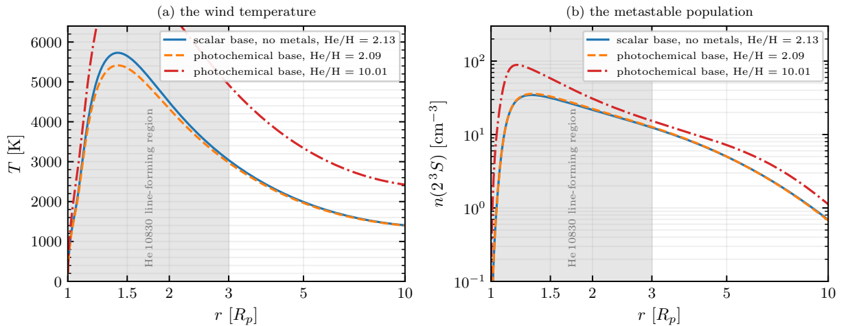
Figure 17: The thermostat, on the three solutions of Table 15. (a) temperature and (b) the metastable density, against radius, with the He 10830 line-forming region 1\text{--}3R_p shaded. Adding the photochemical column's C, N and O at fixed reservoir (solid to dashed) now costs the wind 315 K in T_{\text{max}} and leaves the metastable population where it was, to within 2 per cent in the peak and in the column. Raising the reservoir on that same base (dashed to dot-dashed) reheats it by 2267 K and lifts the metastable peak by 2.5.
