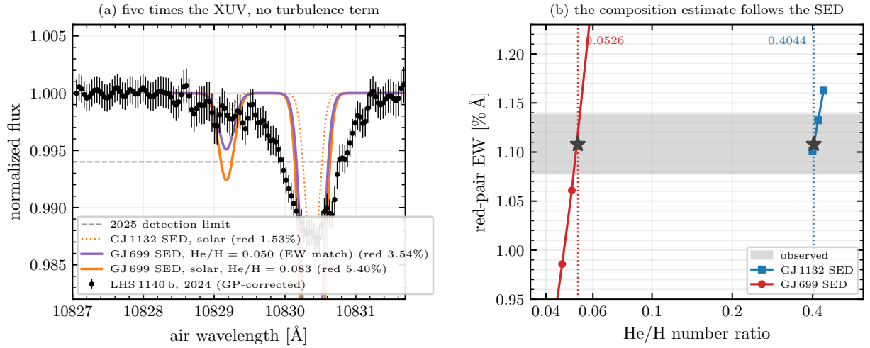
Figure 13: The GJ 699 proxy, five times the XUV of the GJ 1132 proxy used elsewhere in this memo. Left: the measurement with the EXHALE solution nearest the equivalent-width crossing 0.0526, the one at \text{He}/\text{H} = 0.050 , and the solar case on this spectrum, with the GJ 1132 solar case dotted for contrast; all curves without the turbulence term and shifted by the fitted v_{\text{wind}} = +2.26 \text{ km s}^{-1} . The lines are deeper but no wider, the GJ 699 solar curve reaching 3.5\times the depth of the GJ 1132 one (5.40% against 1.53%) while the added broadening the measurement demands of the two differs by 0.45 \text{ km s}^{-1} , or 2 per cent (21.95 against 22.40 \text{ km s}^{-1} ). Right: red-pair equivalent width against composition for the two spectra, with the measured band and the two crossings; the composition the line implies moves from 0.4044 to 0.0526 when the assumed spectrum is changed.
