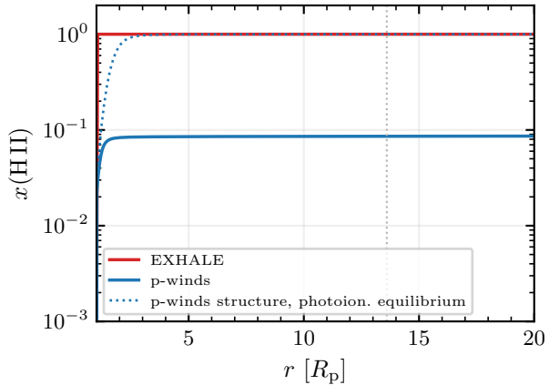
(b) hydrogen ionization
