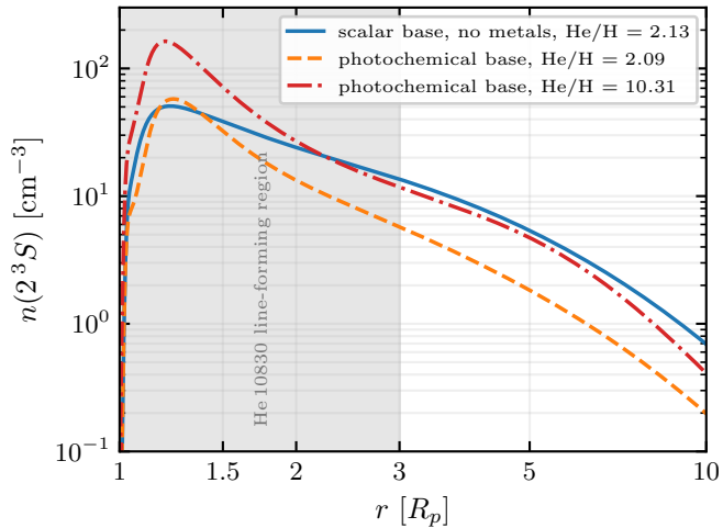
(b) the metastable population
