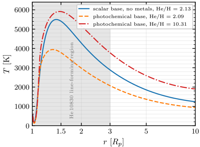
(a) the wind temperature
