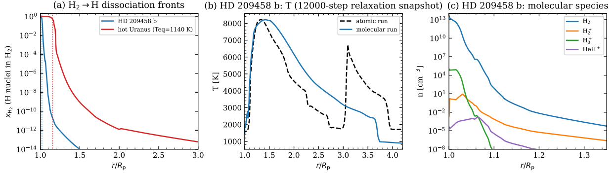
Figure 1: Tier-2 molecular gates (12000-step relaxation snapshots). (a) The H nuclei fraction bound in H_2 : on HD 209458 b the base is fully molecular and a sharp H_2 \rightarrow H front sits at r = 1.020R_p (dotted); on the cooler, low-gravity hot Uranus the front sits at 1.156R_p . The cell-to-cell flip-flop just above the front marks the chemically bistable zone of equilibrium H_2 chemistry — kinetics+advection smooth it (the documented Tier-2 caveat). (b) The molecular run’s temperature agrees with the atomic run away from the (still-relaxing) front region. (c) Molecular species on HD 209458 b: H_3^+ (green) and the molecular ions are confined below the front, as expected for a hot Jupiter.
