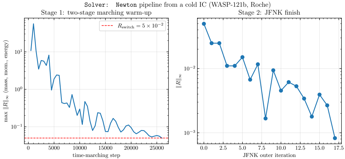
Figure 1: The Solver: Newton pipeline from a cold IC (WASP-121b, Roche). Left: maximum steady residual \max \|R\|_\infty over the mass, momentum, and energy equations during the two-stage (Reconstruction scheme: PLM+WENO3) marching warm-up; the dashed line is the legacy residual hand-off threshold R_{\text{switch}} = 5 \times 10^{-2} used when this figure was produced (the current default keys the hand-off on du < 10^{-2} instead, at a comparable point on the warm-up). Right: residual vs. JFNK outer iteration during the Newton finish, down to \text{Resid tol} ( 10^{-3} ).
