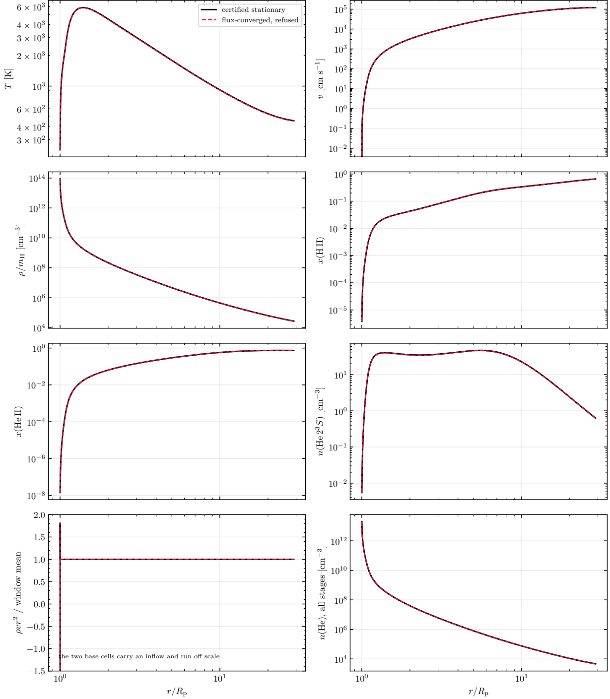
Figure 4: The certified stationary solution and the flux-converged refused state of the atomic scalar_gj1132_kzz1e9/HeH2.13, as functions of radius. The last panel is the number density of all helium nuclei, He I + He II + He III, independent of ionization and level.
