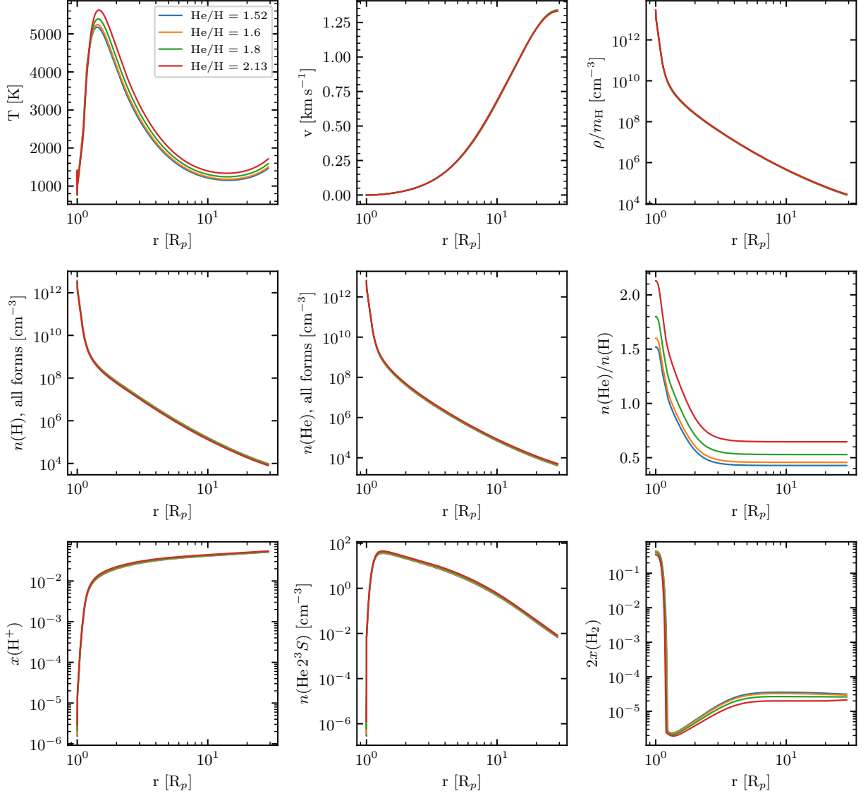
Figure 3: The certified molecular K_{zz} = 10^9 states He/H = 1.52 to 2.13 under the corrected atomic physics (advection-corrected profiles): temperature, velocity, \rho/m_H , the number densities of all hydrogen nuclei n(H) and all helium nuclei n(He) (every ionization stage, level and molecule counted: H I, H II, 2 H_2 , 2 H_2^+ , 3 H_3^+ and HeH^+ for hydrogen; He I, He II, He III and HeH^+ for helium), their ratio n(He)/n(H) , the H II fraction, n(He 2^3 S) and the H 2 fraction against radius.
