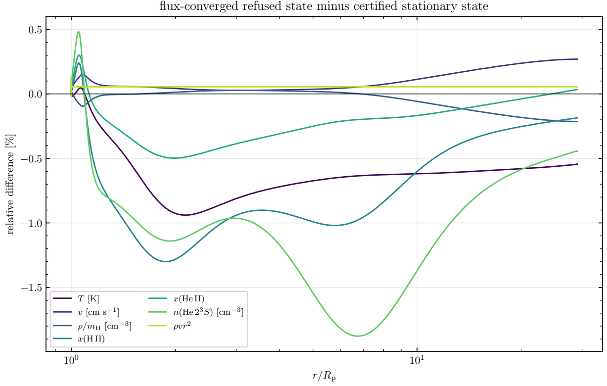
Figure 5: The same two states, as the relative difference of each quantity. The largest are the temperature at r = 2.13 R_p ( -0.94 per cent), x(\text{He II}) at 1.87 ( -1.30 ) and n(\text{He } 2^3S) at 6.74 ( -1.88 ).
