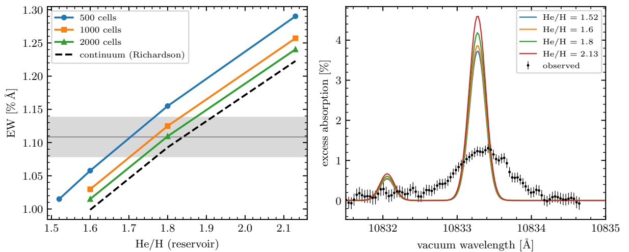
Figure 1: Left: the red-pair EW of the certified molecular states against the reservoir He/H on 500, 1000 and 2000 cells and in the continuum limit, with the observed 1.108 \pm 0.030 \text{ \% Å} (grey). Right: the unbroadened 500-cell spectra against the released one.
