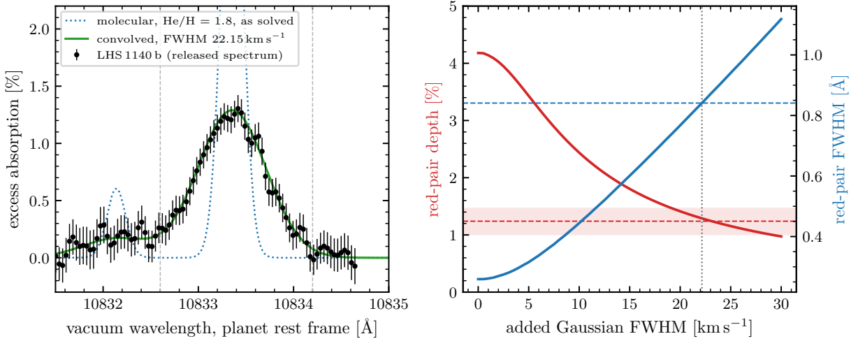
Figure 2: Left: the molecular \text{He}/\text{H} = 1.8 profile as solved (dotted) and convolved with a 22.15 \text{ km s}^{-1} FWHM Gaussian (solid), against the released spectrum; both model curves are shifted by the memo’s v_{\text{wind}} = +2.26 \text{ km s}^{-1} for display (every EW is from the unshifted arrays), and the dashed verticals mark the EW window. Right: the red-pair depth (red, left axis) and FWHM (blue, right axis) as the added Gaussian is scanned; dashed lines are the observed values, the band the 1\sigma interval of the fitted depth, and the dotted vertical the matched kernel.
