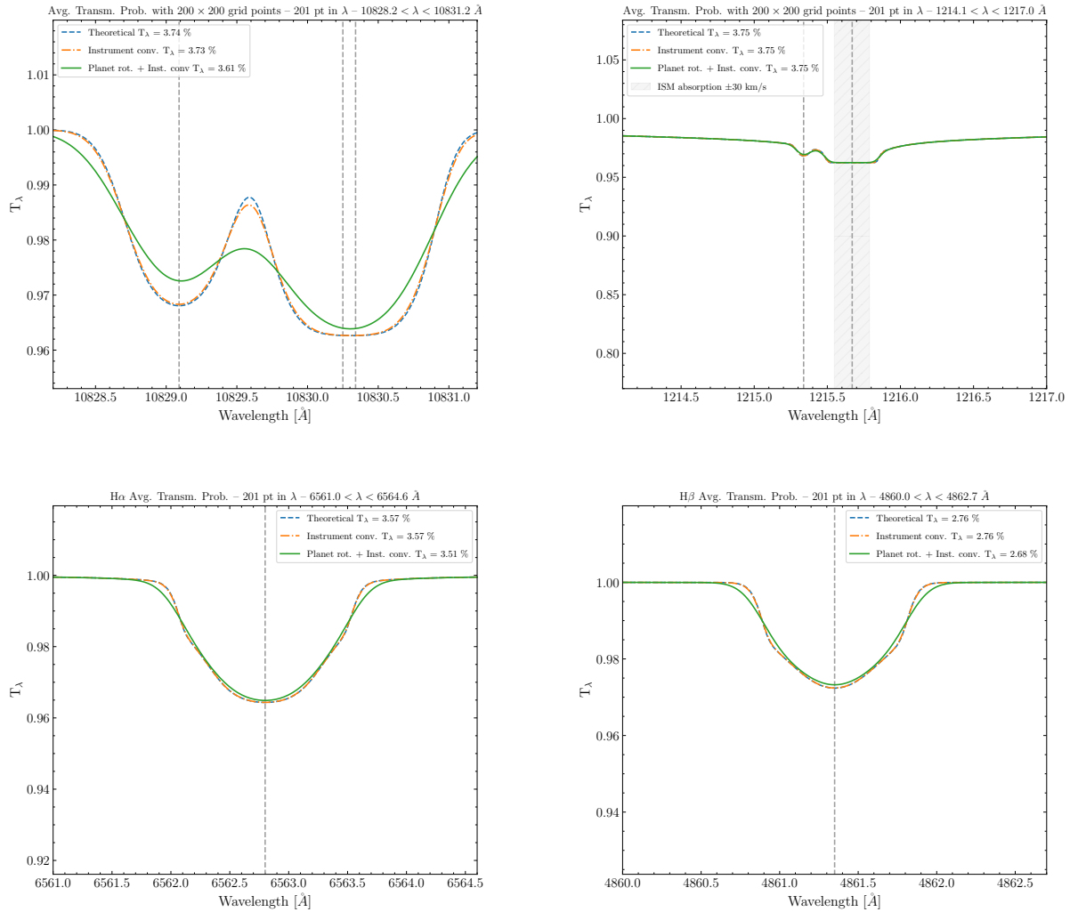
Figure 2: TPM.py output spectra for WASP-121b (Roche, Newton solution with He 2 3 S on; regression/tpm_wasp/ ): He I 10830 (top left), Ly \alpha (top right), H \alpha (bottom left), and H \beta (bottom right). Each panel shows the theoretical line, the instrument-convolved line, and the instrument+rotation-convolved line as produced by the script.
