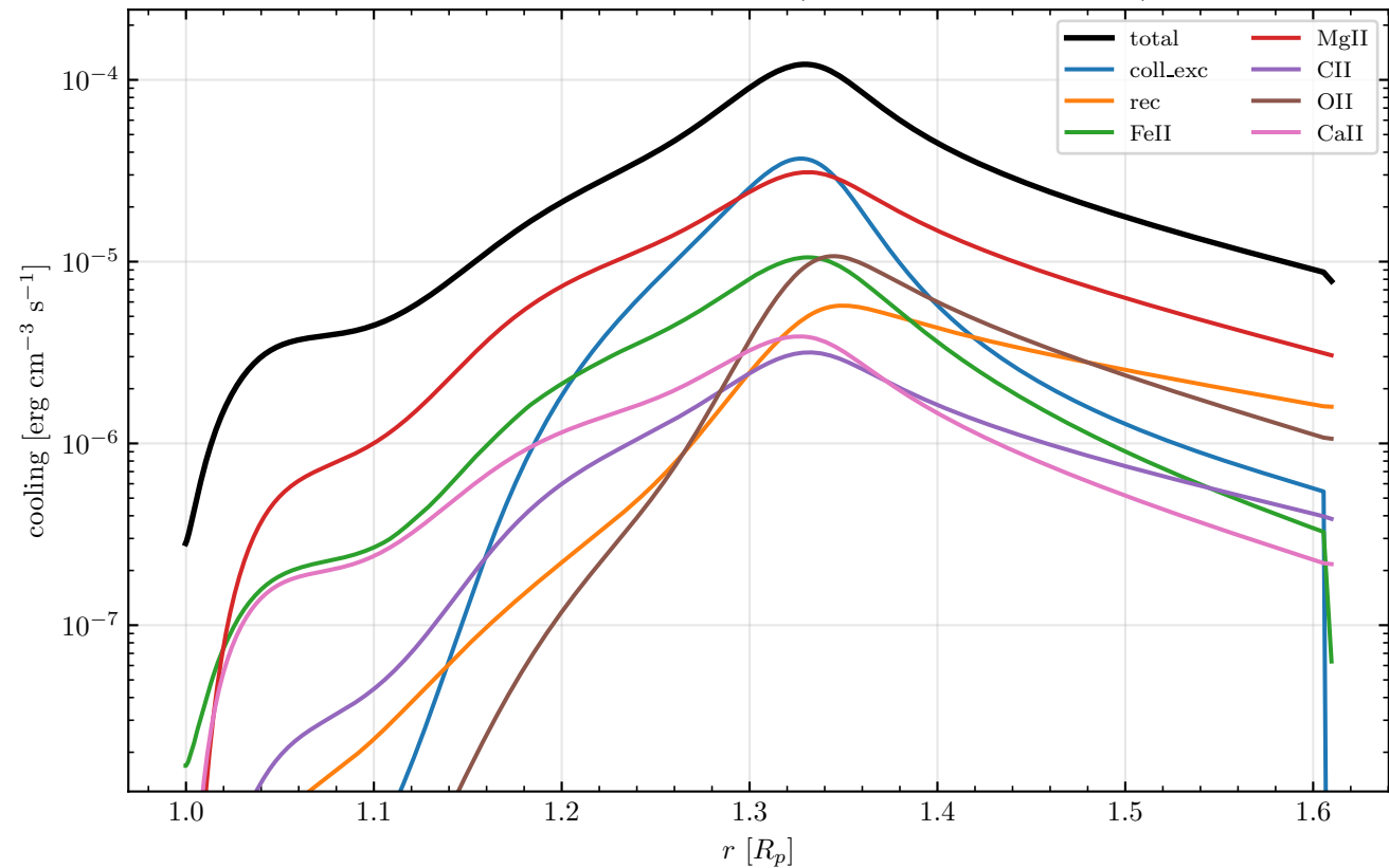
Per-channel radiative cooling (WASP-121b, metals on)
