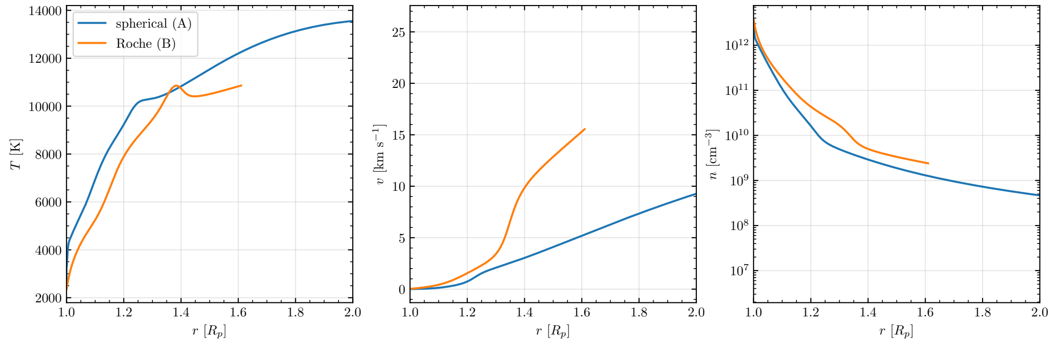
Spherical vs. Roche (RLOF): \dot{M}_A = 0.053 , \dot{M}_B = 0.340 \ M_p/\text{Gyr}
