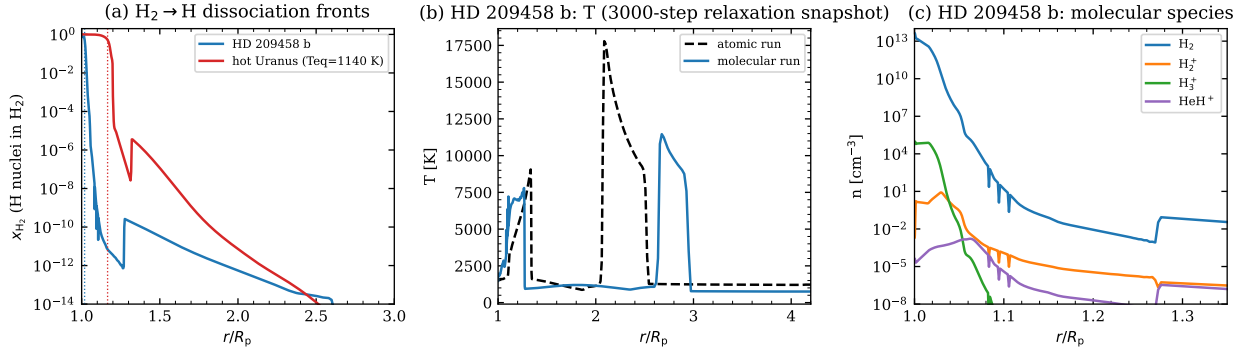
Figure 1: Tier-2 molecular gates (3000-step relaxation snapshots). (a) The H nuclei fraction bound in H 2 : on HD 209458 b the base is fully molecular and a sharp H 2 → H front sits at r = 1.019 R_p (dotted); on the cooler, low-gravity hot Uranus the front rises to 1.166 R_p . The cell-to-cell flip-flop just above the front marks the chemically bistable zone of equilibrium H 2 chemistry — kinetics+advection smooth it (the documented Tier-2 caveat). (b) The molecular run’s temperature agrees with the atomic run away from the (still-relaxing) front region. (c) Molecular species on HD 209458 b: H 3 + (green) and the molecular ions are confined below the front, as expected for a hot Jupiter.
