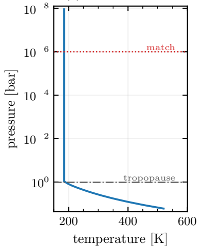
(b) the solved climate
