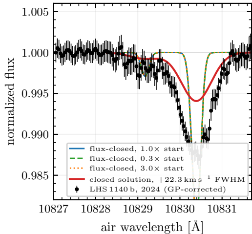
(a) the line at the flux-closed composition
