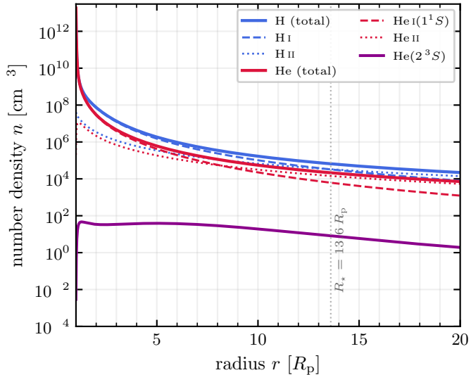
(a) H and He number densities ( K_{zz} = 10^9 , He/H = 1.6108)
