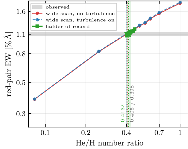
Figure 4: Red-pair equivalent width against composition, with and without the turbulence term, against the measured band. The crossing is insensitive to the broadening treatment: all seven arms of this scan were re-solved on the current binary and each was synthesized twice (LHS1140b/exhale/refresh_j96/scan/), so both curves stand on one physics, and they cross the measured band at \text{He}/\text{H} = 0.4051 without the turbulence term and 0.3982 with it, 1.7 per cent apart. The crossing this memo quotes for this axis, 0.4132 , is the one of Sect. 7., read off the ten-arm ladder whose spacing brackets the measurement four times more closely; this scan reproduces it to 2.0 per cent.
