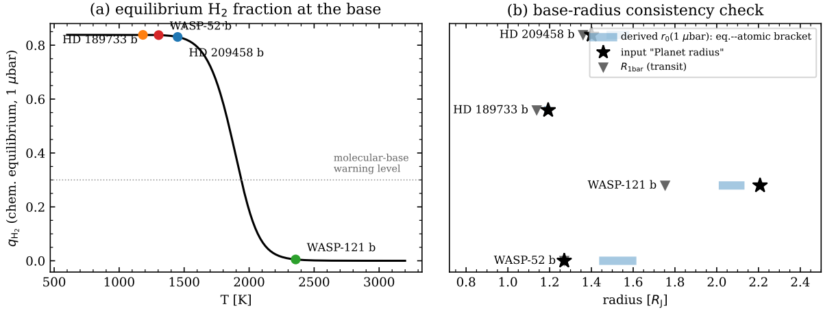
Figure 3: Tier-1 analytic column applied to the four planets. (a) The chemical-equilibrium H_2 mixing ratio at 1 \mu\text{bar} (Eq. 2) as a function of temperature: the three T_{\text{eq}} \lesssim 1500 K planets sit on the fully molecular plateau, while WASP-121 b ( T_{\text{eq}} = 2358 K) is atomic even in equilibrium. (b) Derived 1- \mu\text{bar} base radius (equilibrium-atomic bracket, shaded) versus the production “Planet radius” (star) and the transit radius (triangle): HD 189733 b falls inside its bracket, HD 209458 b sits \sim 5\% below, WASP-121 b lies just above (dayside-hot lower atmosphere), and WASP-52 b’s transit-radius shortcut puts the base 0.17–0.35 R_J too deep.
