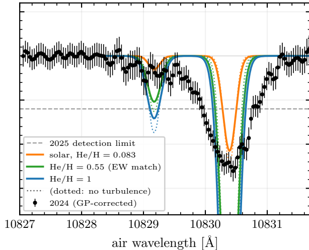
(b) EXHALE, wind solved; solid: turbulence on
