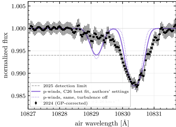
(a) p-winds at the C26 best fit (MCMC medians)
