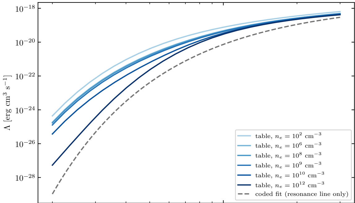
Mg I line cooling per n_e n_{\text{ion}}
