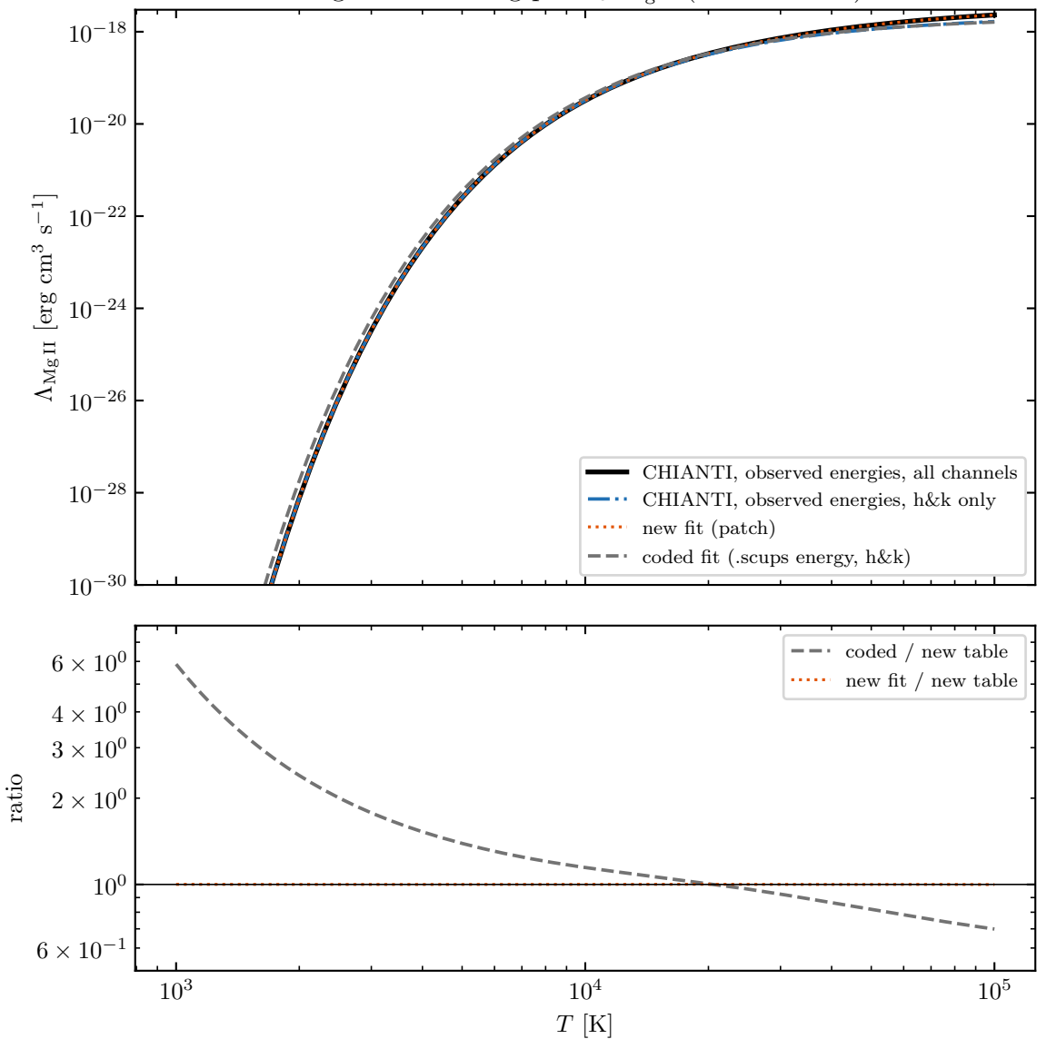
Mg II line cooling per n_e n_{\text{Mg II}} (coronal limit)
