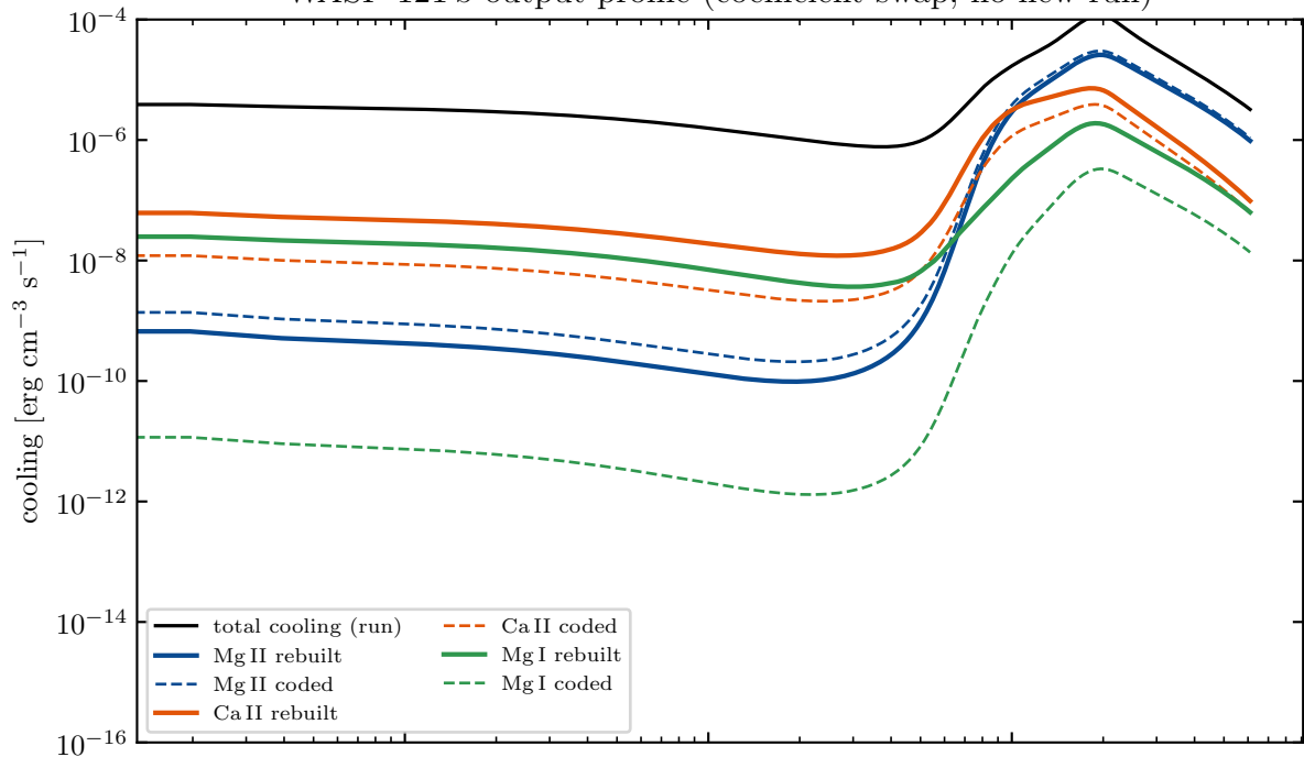
WASP-121 b output profile (coefficient swap, no new run)
