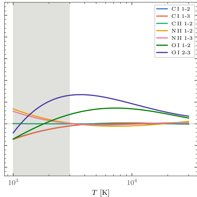
ground-term fine-structure \Upsilon
