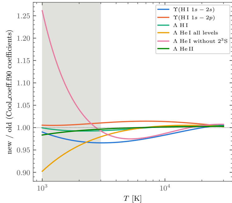
H and He excitation
