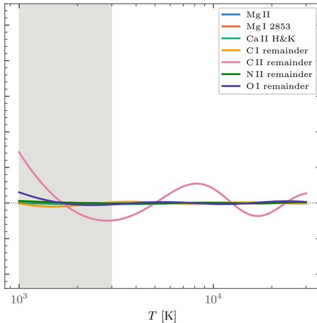
metal resonance and remainder fits
