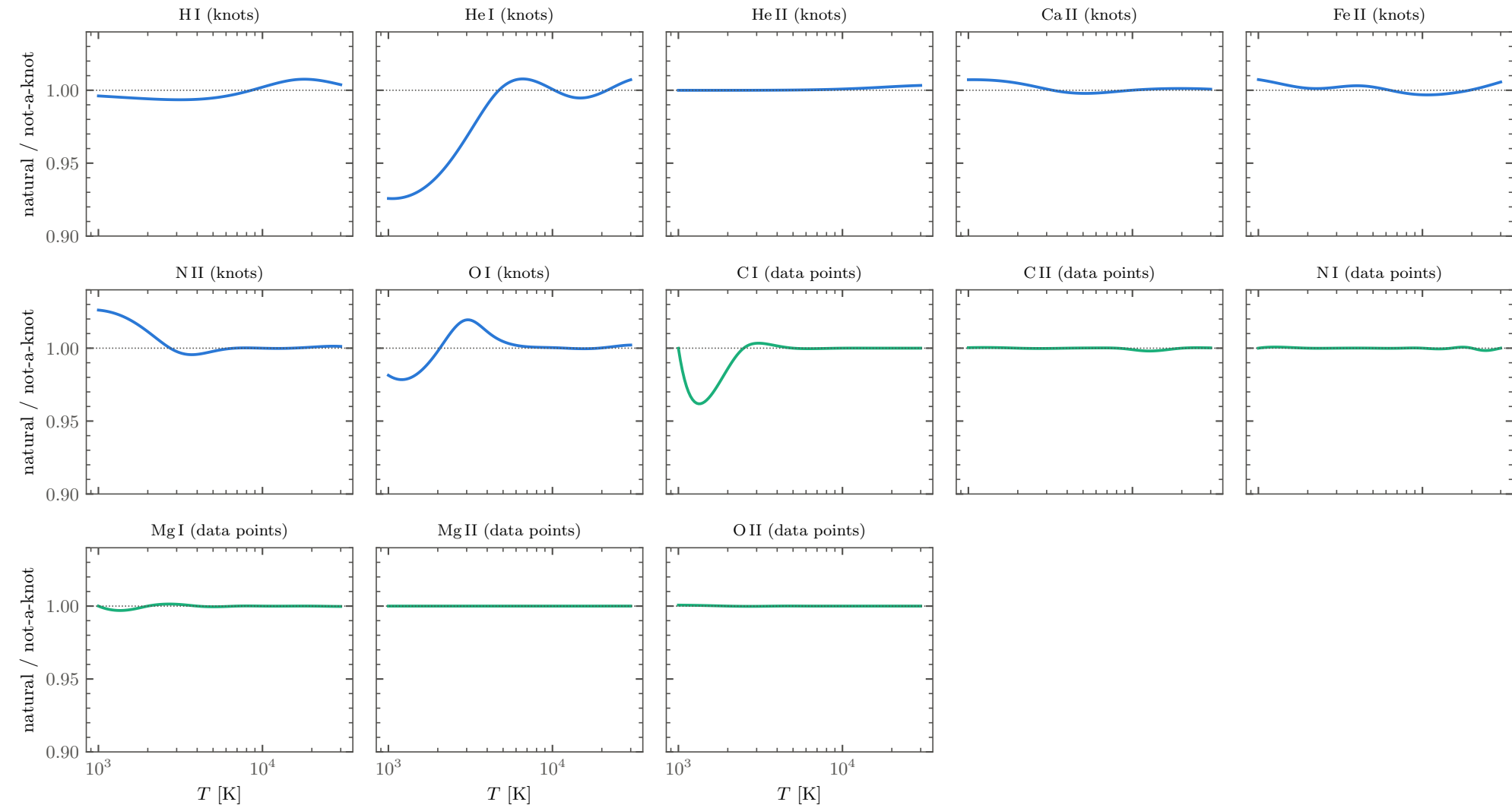
Coronal ground-level line cooling \sum_u q_{1u} E_{1u} , CHIANTI v11.0.2, observed energies
